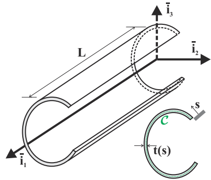
Fig. 8.2. Thin-walled beam with an open section.
