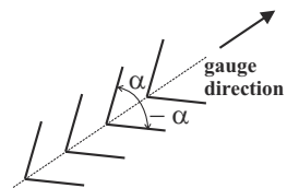
Fig. 2.4. Configuration of the “fish-bone” gauge.
