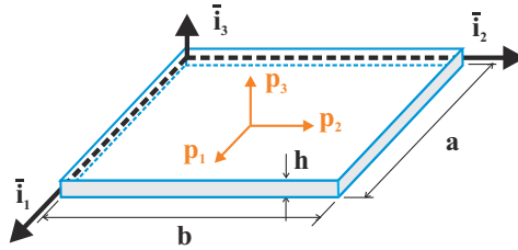
Fig. 16.1. Rectangular plate of thickness h .
