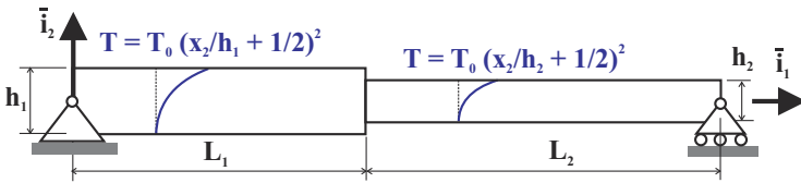
Fig. 13.24. Simply supported beam subjected to parabolic thermal gradients.
