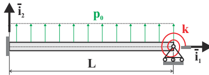
Fig. 11.15. Cantilevered beam with tip support and rotational spring under uniform load.
