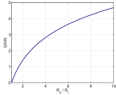
Fig. 13.6. Gain in maximum pressure for a fully plastic tube as compared to the tube operating entirely in the elastic regime.
