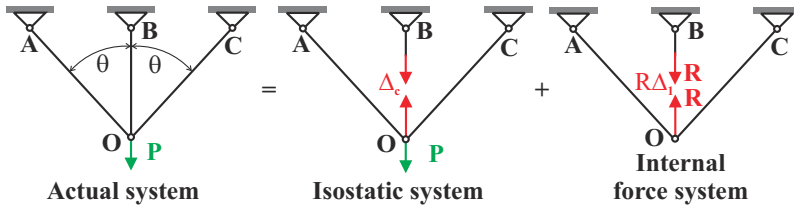
Fig. 9.66. Force method for the three-bar truss.
