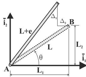
Fig. 9.29. Single bar of a planar truss.
