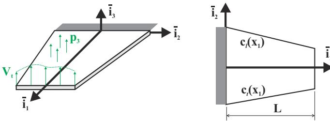
Fig. 16.44. Wing modeled as a thin flat plate.
