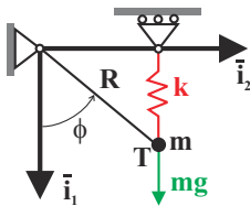
Fig. 9.14. Rotating mass with vertical spring.
