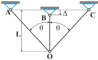
Fig. 10.28. Three-bar truss with prescribed displacement.
