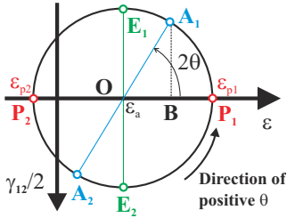
Fig. 1.23. Mohr's circle for visualizing plane strain state.
