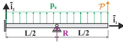
Fig. 10.47. Application of Castigliano's second theorem to calculate deflections in a hyperstatic beam.
