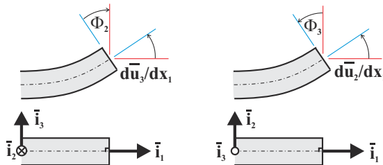
Fig. 5.4. Beam slope and cross-sectional rotation.
