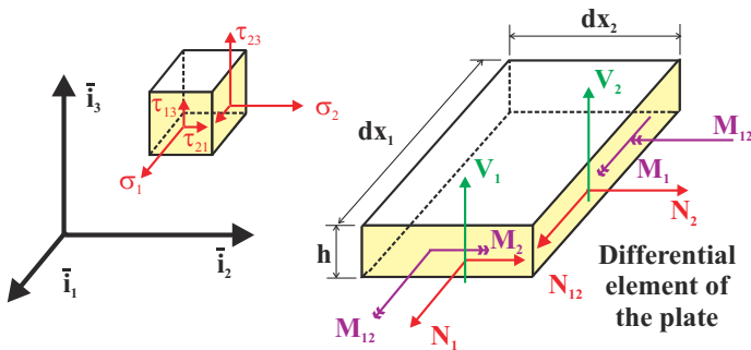
Fig. 16.3. Stress resultants acting on a differential element of the plate.
