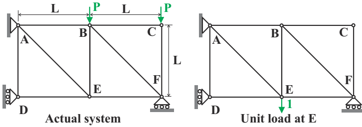
Fig. 9.69. Deflection of a joint in a two-bay truss with a redundant support.
