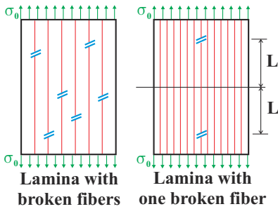
Fig. 2.12. Lamina with a broken fiber.
