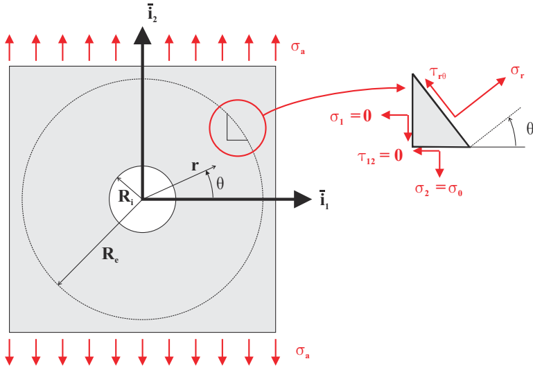
Fig. 3.12. Thin sheet with central hole of radius R_i subjected to uniaxial stress \sigma_2 = \sigma_a ; also shown is the far field circle at r = R_e where boundary conditions are applied.
