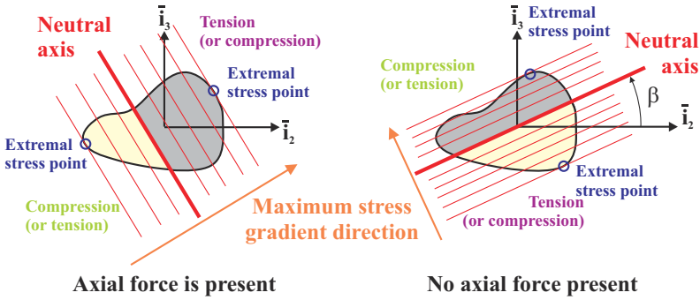
Fig. 6.6. Neutral axis on a cross-section: left portion, axial force is preset, right portion, the axial force vanishes. Along the red lines, the axial stresses remain constants.
