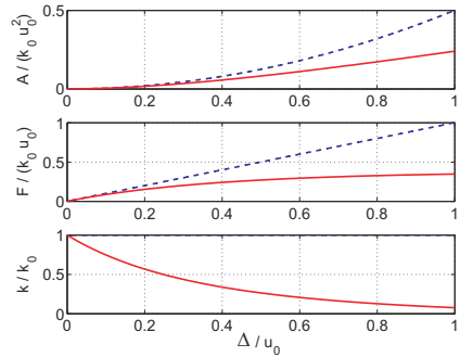
Fig. 10.8. Nonlinear “bungee” spring with the potential given by eq. (10.27). Top figure: strain energy; middle figure: force; bottom figure: stiffness. Solid line: nonlinear spring; dashed line: linear spring.
