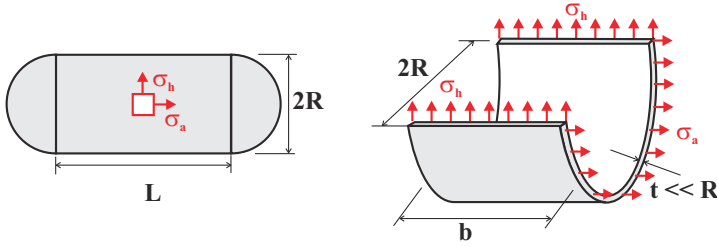
Fig. 1.14. Long, thin-walled cylindrical pressure vessel (left) and free body diagram (right) used to calculate in-plane stresses \sigma_h and \sigma_a .
