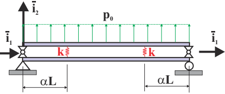
Fig. 11.38. Two simply supported beams with interconnecting springs.
