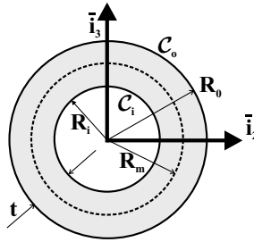
Fig. 7.20. Cross-section of a circular tube.
