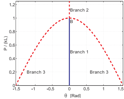
Fig. 10.13. Response of the system: stable branch: solid line; unstable branches: dotted lines.
