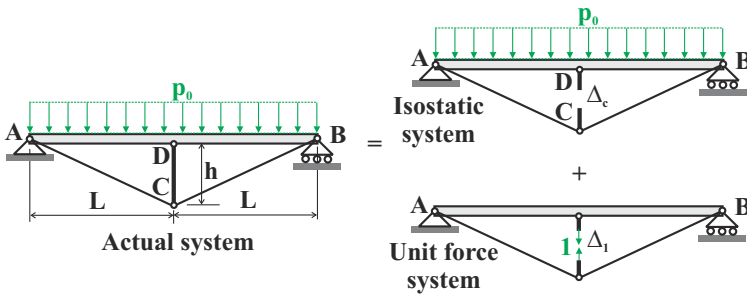
Fig. 9.74. Calculation of bending moment distribution in beam and forces in bars in a hyperstatic beam-truss problem.
