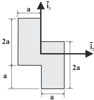
Fig. 6.20. Double-rectangular section.
