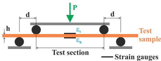
Fig. 5.19. Configuration of the four-point bending test.
