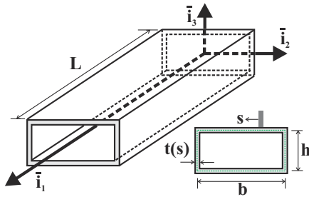
Fig. 8.1. Thin-walled beam with a closed, single cell section.
