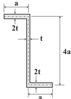
Fig. 6.25. Reversed “Z” shaped cross-section.
