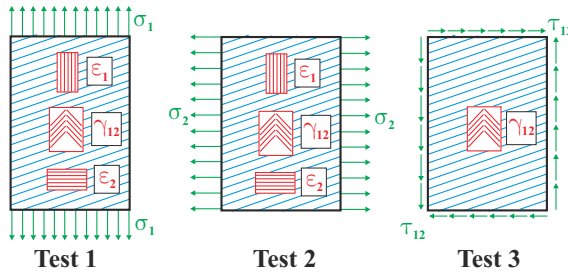
Fig. 2.22. Three simple tests for the determination of the engineering constants.
