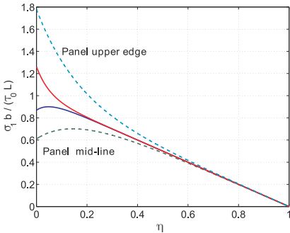
Fig. 12.9. Distribution of axial stress along the panel span. Isotropic material: solid line; anisotropic material: dashed line.
