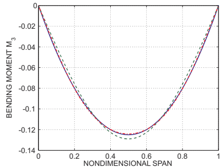
Fig. 11.27. Bending moment M_3 versus non-dimensional span. Exact solution: solid line; Approximate solution: dashed line (case 1), dash-dotted line (case 2).
