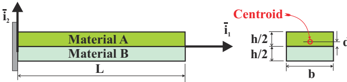
Fig. 13.22. Cantilevered bi-material beam under uniform temperature field.
