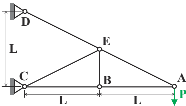
Fig. 9.46. Planar truss with tip load.
