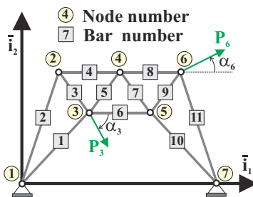
Fig. 10.22. Eleven-bar truss with node and element numbering.
