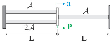
Fig. 4.9. Three bars in a parallel-series configuration.
