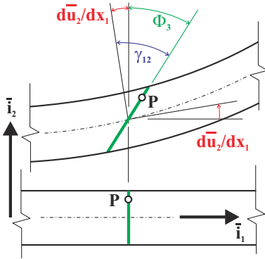
Fig. 15.8. Kinematic assumptions for shear deformable beams.
