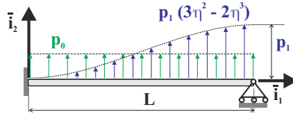
Fig. 11.11. Cantilever beam with tip support subjected to two different loading conditions.
