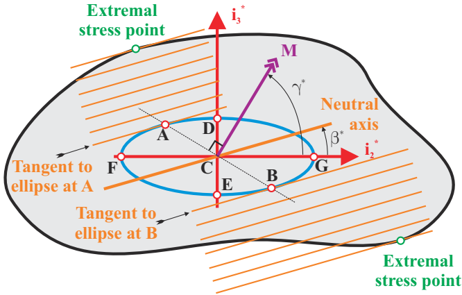
Fig. 6.7. Cross-section subjected to a bending moment, M .
