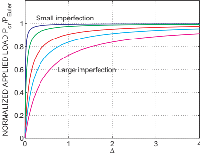
Fig. 14.9. Mid-span transverse deflection of an imperfect pinned-pinned beam for various levels of imperfection.
