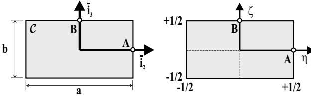
Fig. 7.21. Bar with a rectangular cross-section.
