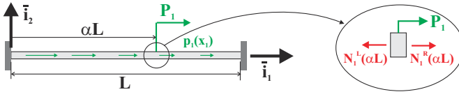
Fig. 11.17. Beam fixed at both ends and subjected to distributed axial load and concentrated load.
