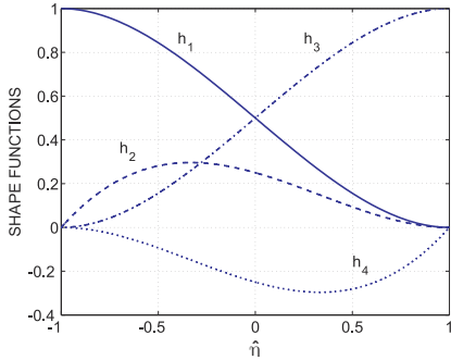
Fig. 11.45. Beam element shape functions. h_1 : solid line; h_2 : dashed line; h_3 : dash-dotted line; h_4 : dotted line.
