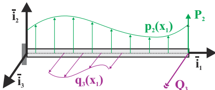
Fig. 12.12. Cantilevered beam with concentrated and distributed moments.
