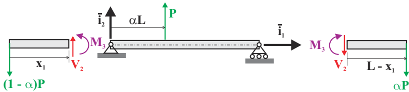
Fig. 5.24. Simply supported beam with one concentrated load.
