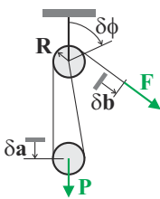
Fig. 9.10. Simple two-pulley block and tackle system.
