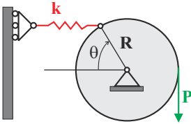
Fig. 9.17. Rotating disk with spring restraint.
