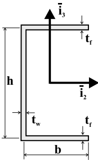
Fig. 7.32. A thin-walled C-channel section
