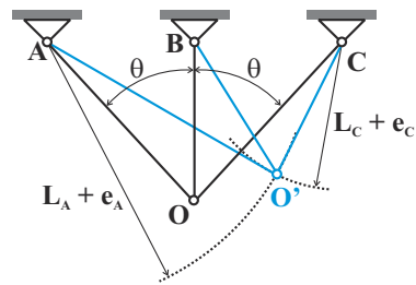
Fig. 9.35. Three-bar truss in the original and deformed configurations.
