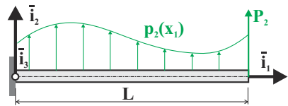
Fig. 12.5. Cantilevered beam with distributed transverse load.
