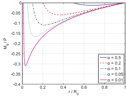
Fig. 16.35. Radial distribution of non-dimensional bending moments, M_\theta / P .
