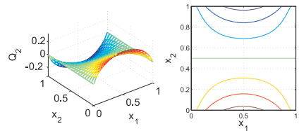
Fig. 16.28. Distribution of transverse shear force, Q_2 , over the plate.
