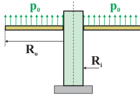
Fig. 16.38. Circular plate clamped to a center rigid shaft.
