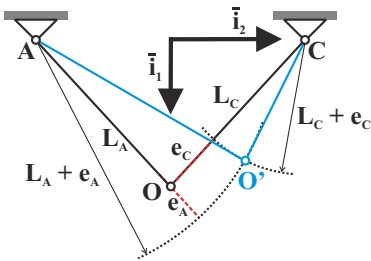
Fig. 9.34. Two-bar truss in the original and deformed configurations.
