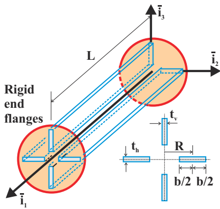
Fig. 8.63. Configuration of the four-web flexure.
