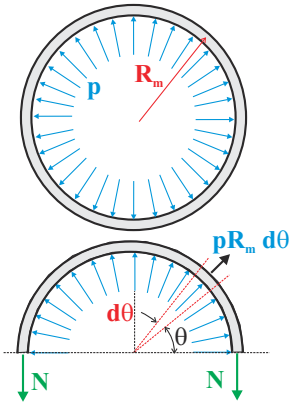
Fig. 3.10. Thin ring under internal pressure.
