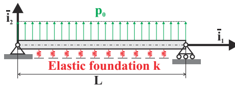
Fig. 5.32. Simply supported beam on an elastic foundation.
