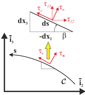
Fig. 7.16. Equilibrium condition along the outer contour C .
