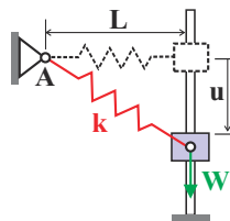
Fig. 9.22. Mechanism with nonlinear geometry.
