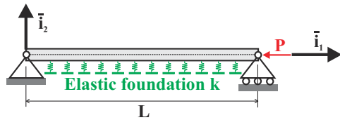
Fig. 14.28. Upper face of a sandwich structure under end compressive loads. The core of the sandwich is modeled by an elastic foundation.
