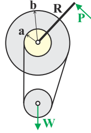
Fig. 9.24. Differential pulley with an applied moment.
