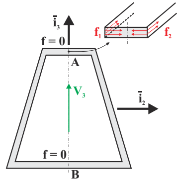
Fig. 8.34. Trapezoidal section subjected to a shear force.
