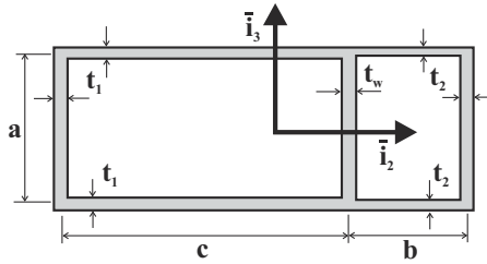
Fig. 8.45. Thin-walled beam with two cells.
