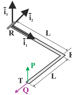
Fig. 9.62. Beam under combined bending and torsion.
