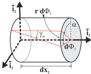
Fig. 7.4. Visualization of out-of-plane shear strain in polar coordinates.
