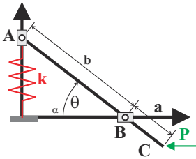
Fig. 10.14. Lever with spring-restrained sliding pivots.
