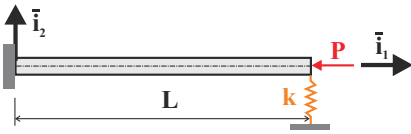
Fig. 14.22. Cantilevered beam with tip spring.
