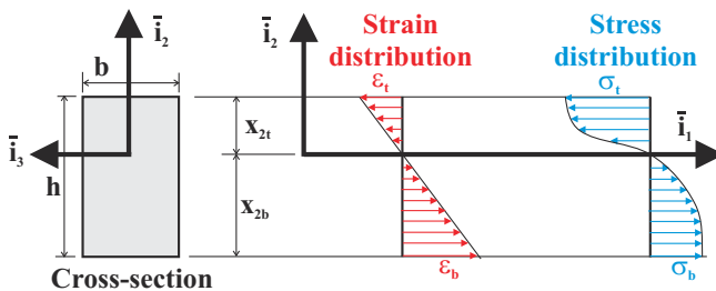
Fig. 13.7. Beam with a rectangular cross-section undergoing plastic bending.
