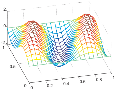
Fig. 16.56. Assumed deflection for shear buckling of long plate ( m = 3 ).
