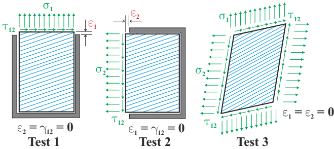
Fig. 2.23. Three simple tests for the determination of the stiffness coefficients.
