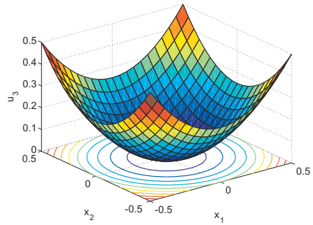
Fig. 16.12. Transverse displacement distribution for synclastic bending.
