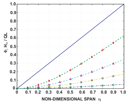
Fig. 8.77. Twist distribution for the C-channel section under non-uniform torsion. \bar{k} = 2.65 ( \diamond ), \bar{k} = 1.33 ( \triangle ), \bar{k} = 0.808 ( \square ), \bar{k} = 0.404 ( \circ ).
