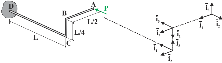
Fig. 9.54. Bent beam assembly under tip load.
