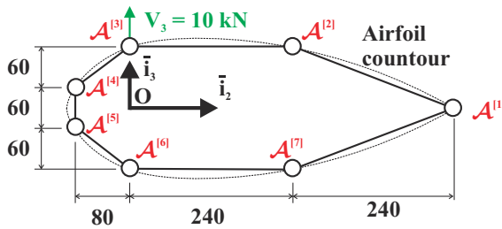
Fig. 8.84. Sheet-stringer model for wing cross-section (dimensions in mm).
