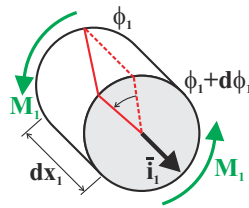
Fig. 9.49. Torsional deformation of an infinitesimal segment of a beam.
