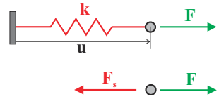
Fig. 10.4. Rectilinear spring subjected to a force F .
