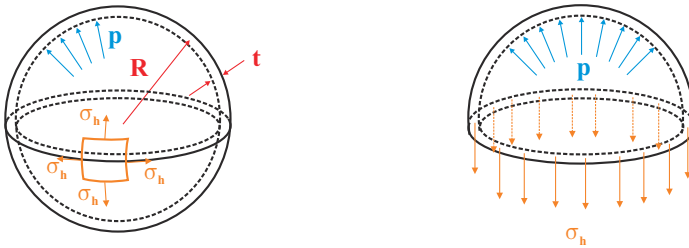
Fig. 3.16. Thin sphere under internal pressure.
