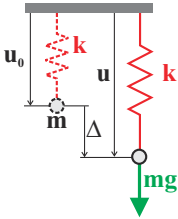
Fig. 10.10. Rectilinear spring supporting a weight.
