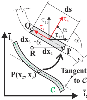
Fig. 8.5. Geometry of a differential element of the wall.
