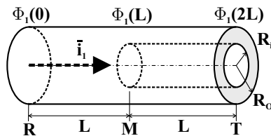
Fig. 7.9. Circular bar with hollow segment.
