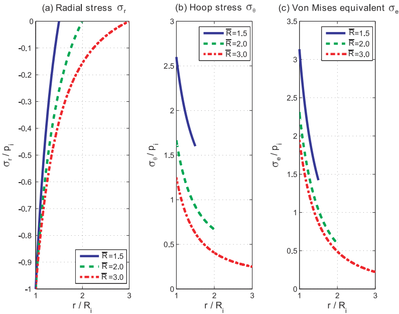
Fig. 3.8. Plots of the non-dimensional radial stress, \sigma_r/p_i , hoop stress, \sigma_\theta/p_i , and Von Mises' equivalent stress, \sigma_e/p_i , for three different thickness ratios \bar{R} = 1.5, 2.0, 3.0 .
