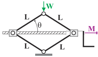
Fig. 9.27. Screw jack type of scissor lift.
