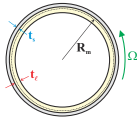
Fig. 4.19. Configuration of the bi-material fly wheel.
