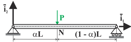
Fig. 10.49. Simply-supported beam under concentrated load
