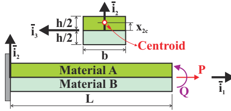
Fig. 5.48. Cantilevered bi-material beam under tip loads.
