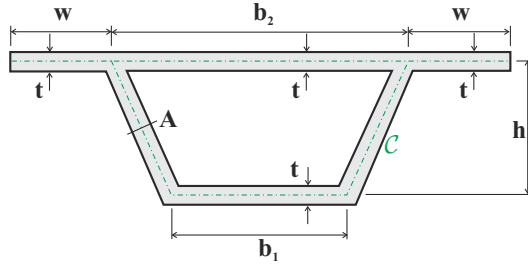
Fig. 8.52. Thin-walled trapezoidal beam with overhangs.
