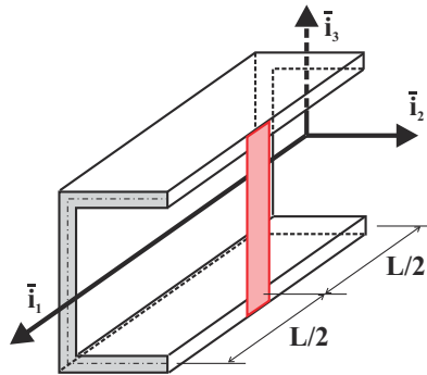
Fig. 8.78. Cantilevered beam with C-section with a mid-span reinforcing plate.
