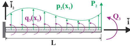
Fig. 15.7. Cantilevered beam under distributed and concentrated transverse loads and bending moments.
