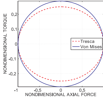
Fig. 7.10. Yield envelopes predicted by Tresca’s and von Mises’ criteria plotted in the non-dimensional loading space.
