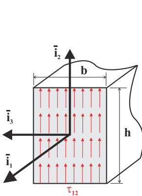
Fig. 1.9. Uniform distribution of shear stresses over the cross-section of a beam.
