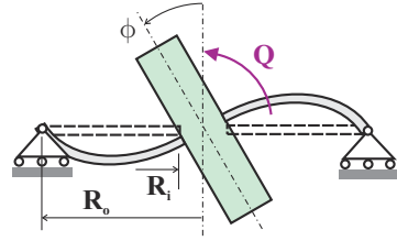
Fig. 16.40. Simply supported circular plate with center rigid shaft.
