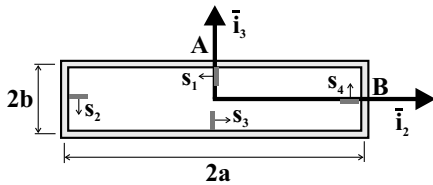
Fig. 12.16. Rectangular cross-section of a thin-walled beam.
