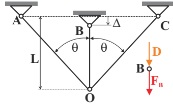
Fig. 9.37. Three-bar truss with prescribed displacement.
