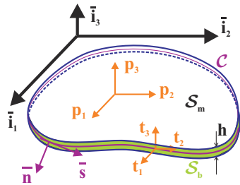
Fig. 16.41. Plate of arbitrary shape.
