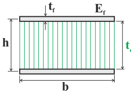
Fig. 14.27. Cross-section of a sandwich beam.
