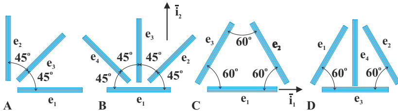
Fig. 1.26. Various commonly used strain gauge arrangements.
