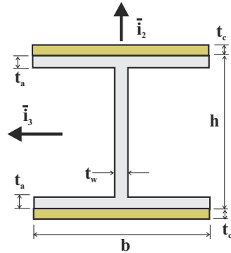
Fig. 5.13. Cross-section of a reinforced I beam.
