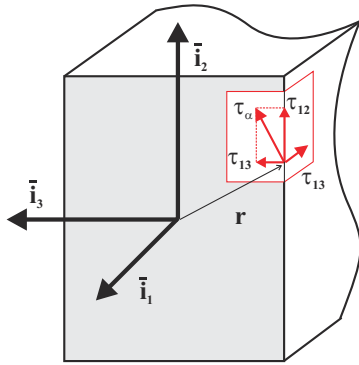
Fig. 7.14. Shearing stresses along the edge of a rectangular section.
