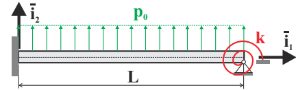
Fig. 10.35. Cantilevered beam with tip rotational spring.
