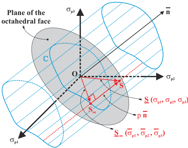
Fig. 13.1. The geometric representation of stress states defined in terms of principal stresses.
