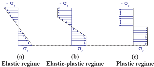
Fig. 13.8. The three regimes of the cross-section: the purely elastic, elastic-plastic, and fully plastic regimes.
