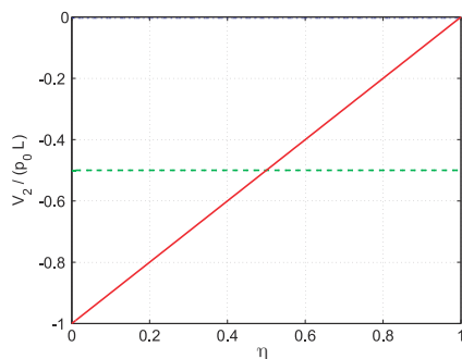
Fig. 11.5. Non-dimensional shear force field for the cantilevered beam. Solid line: three-term polynomial solution (exact solution); dashed line: two-term approximation; dash-dotted line: single-term approximation.
