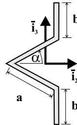
Fig. 8.17. Horizontal “V” section with vertical flanges.
