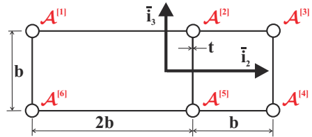
Fig. 8.86. Sheet-stringer beam with two cells.
