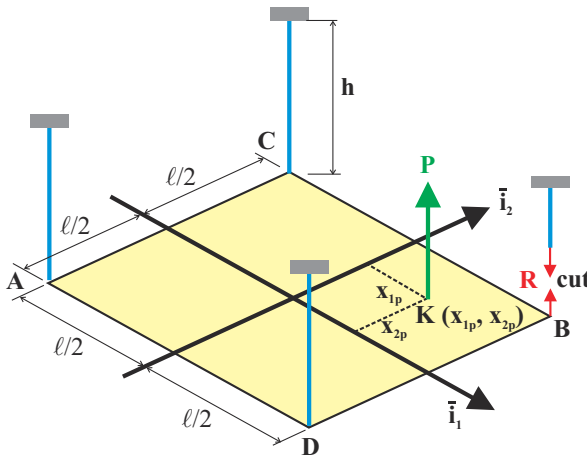
Fig. 4.8. A rigid plate supported by four identical elastic cables.
