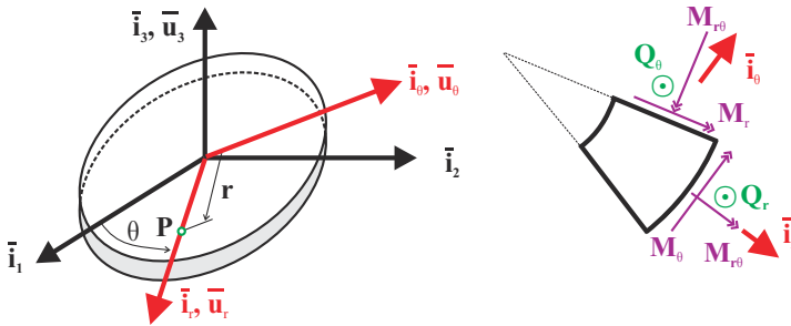
Fig. 16.30. Circular plate with Cartesian and polar coordinate systems.
