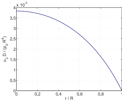
Fig. 16.31. Radial distribution of the non-dimensional displacement, \bar{u}_3 D/(p_0 R^4) .
