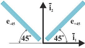
Fig. 1.24. Two strain gauges at the surface of a solid.
