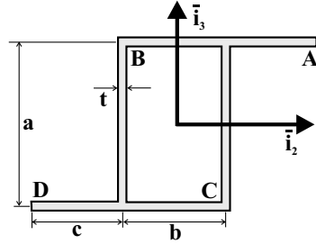
Fig. 8.15. Box-Z shaped cross-section.
