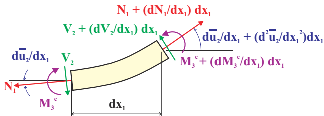
Fig. 14.6. Free body diagram of a deformed slice of the beam.
