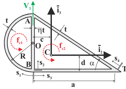
Fig. 8.67. Simplified 2-cell wing cross-section.
