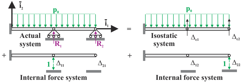
Fig. 9.75. Cantilevered beam with two support.
