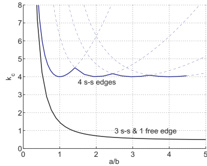
Fig. 16.54. Buckling parameter versus the plate's aspect ratio ( \nu = 0.25 ).
