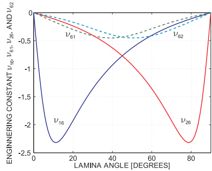
Fig. 2.25. Variation of engineering constants \nu_{16} , \nu_{61} , \nu_{26} , and \nu_{62} with lamina angle \theta .
