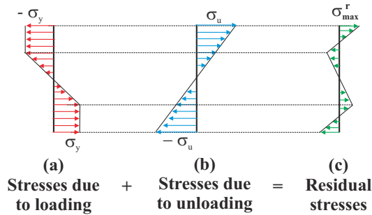
Fig. 13.10. Residual stresses after plastic bending in a section made of elastic-perfectly plastic material.
