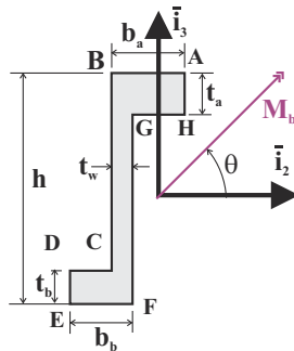
Fig. 6.23. “Z” shaped cross-section.
