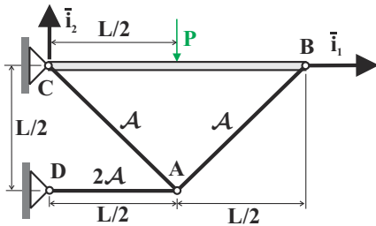
Fig. 9.61. Pivoted beam supported by three-bar truss.
