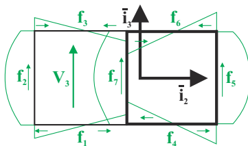
Fig. 8.41. Shear flow in the thin-walled double-box section.
