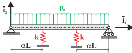
Fig. 5.31. Simply supported beam with two elastic spring supports.
