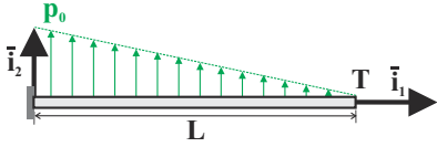
Fig. 9.59. Cantilevered beam subjected to triangular loading.
