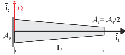
Fig. 11.18. A helicopter blade rotating at an angular speed \Omega .
