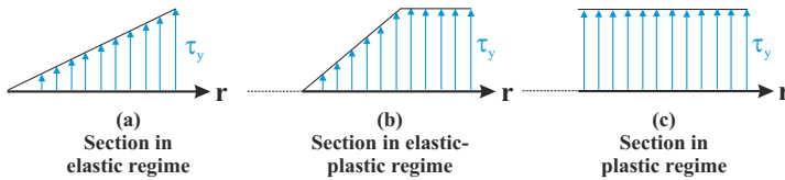
Fig. 13.13. The three stress regimes of the cross-section: (a) purely elastic, (b) elastic-plastic, and (c) fully plastic.
