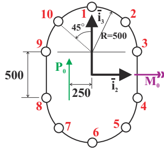
Fig. 8.87. Fuselage sheet-stringer cross-section (dimensions in millimeters).
