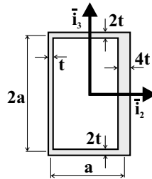
Fig. 8.58. Thin-walled closed rectangular section with variable wall thicknesses.
