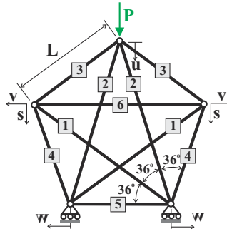
Fig. 10.17. A pentagonal truss.
