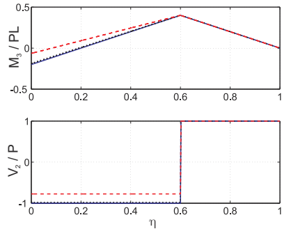
Fig. 15.13. Bending moment (top figure) and shear force (bottom figure) of the cantilevered beam with an intermediate support, \alpha = 0.6 . Shear flexibility parameter \bar{s}^2 = 0 , solid line; \bar{s}^2 = 0.0026 , dotted line; \bar{s}^2 = 0.035 , dashed line.
