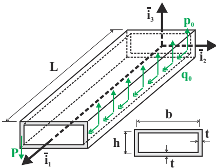
Fig. 8.61. Thin-walled, rectangular box beam.
