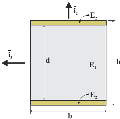
Fig. 5.33. Reinforced rectangular cross-section.
