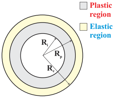
Fig. 13.5. Thick tube under internal pressurization showing the development of concentric plastic and elastic regions.
