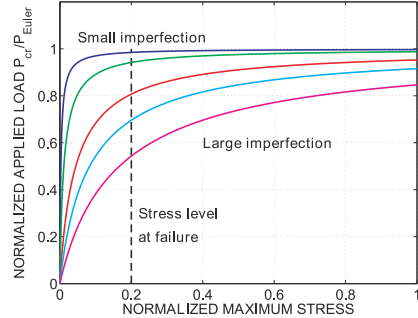
Fig. 14.10. Maximum stress in an imperfect pinned-pinned beam versus applied compressive load.
