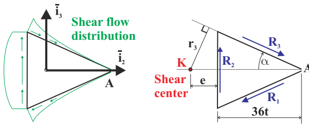
Fig. 8.32. Shear center in thin-walled open triangular section
