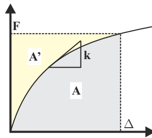
Fig. 10.6. Constitutive law for a nonlinearly elastic spring.
