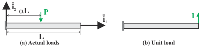
Fig. 9.51. Cantilevered beam under tip load.
