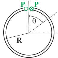
Fig. 10.43. Ring subjected to internal forces acting out of the plane of the ring.
