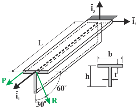
Fig. 6.28. Cantilevered beam with “T” shaped section under tip axial loads.
