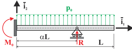
Fig. 10.44. Cantilevered beam with an intermediate support at location \alpha L .
