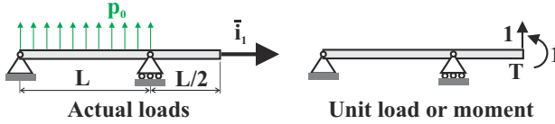
Fig. 9.53. Deflection at tip of a uniformly loaded simply-supported beam with overhang.
