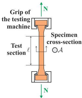
Fig. 2.1. Homogeneous bar loaded by a single stress component \sigma_1
