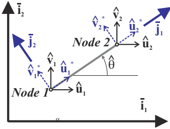
Fig. 10.23. General bar element.
