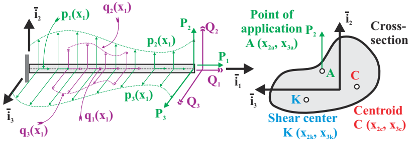
Fig. 8.65. Beam under a complex loading condition.
