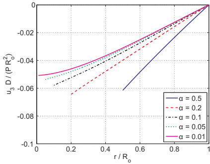
Fig. 16.34. Radial distribution of non-dimensional displacement, \bar{u}_3 D / (P R_o^2) .
