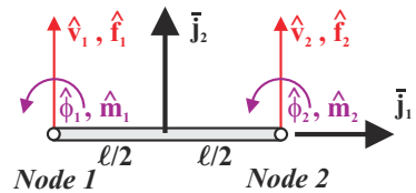
Fig. 11.44. Kinematic of a beam element.
