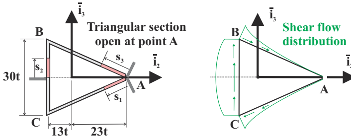
Fig. 8.28. Thin-walled, open triangular section
