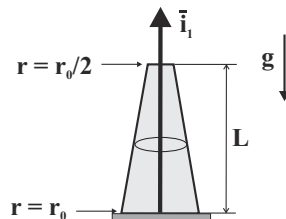
Fig. 11.22. Tapered beam subjected to gravity loads
