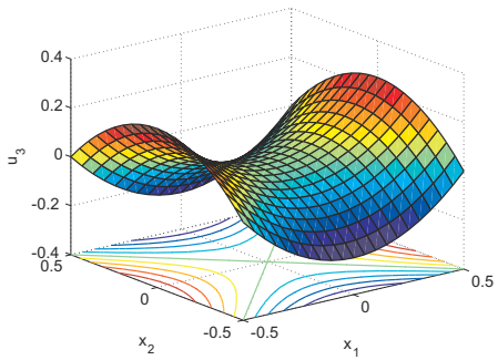
Fig. 16.14. Transverse displacement distribution for anticlastic bending.
