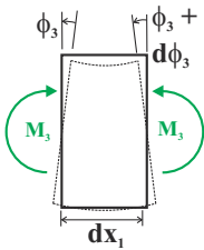
Fig. 9.48. Bending deformation of an infinitesimal segment of a beam.
