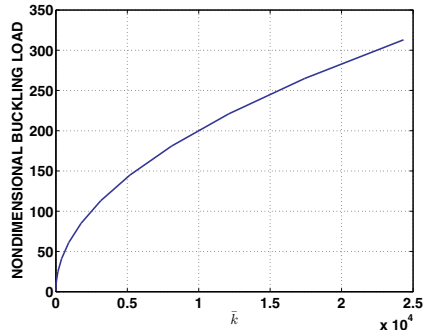
Fig. 14.30. Non-dimensional buckling load P_{cr}/P_{Euler} versus \bar{k} .
