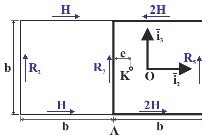
Fig. 8.48. Shear center for a thin-walled double-box section.
