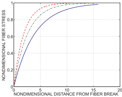
Fig. 2.15. Distribution of fiber axial stress near a fiber break for three material systems.
