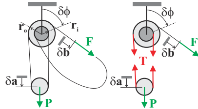
Fig. 9.11. Differential pulley or “chain hoist”.
