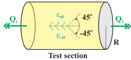
Fig. 7.8. Configuration of the test to determine the torsional stiffness.
