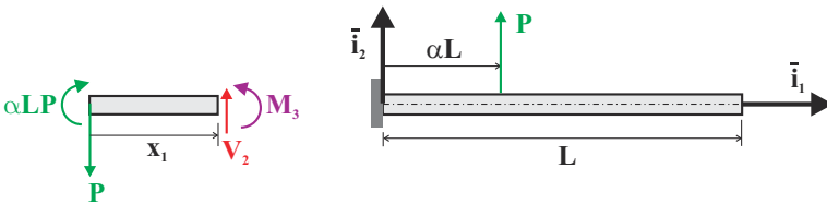
Fig. 5.26. Cantilevered beam under a concentrated load.
