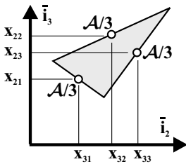
Fig. 6.11. Triangular area equivalent lumped areas.
