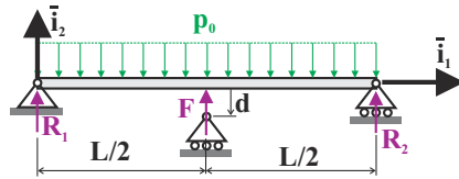
Fig. 10.33. Simply supported beam with a misaligned mid-span support.
