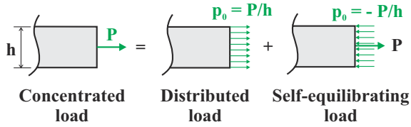
Fig. 4.21. Bar subjected to an end concentrated load.
