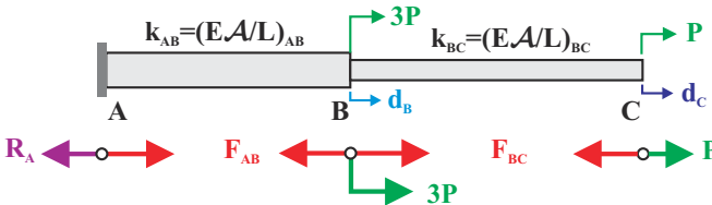
Fig. 4.2. Two bars connected in series and subjected to two loads.
