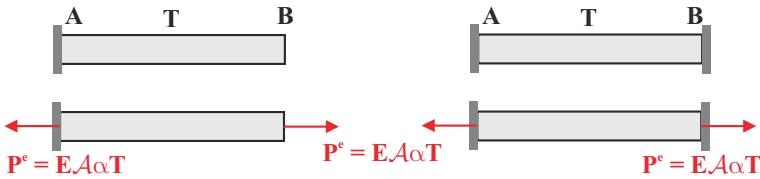
Fig. 13.17. Bar subjected to a uniform temperature. Left figure, the bar is clamped at one end. Right figure, the bar is clamped at both ends.
