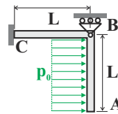
Fig. 9.77. Planar right angle frame with distributed load.
