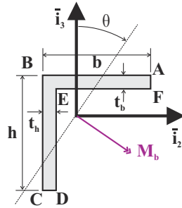
Fig. 6.21. “L” shaped cross-section.
