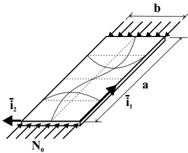
Fig. 16.50. Simply supported plate buckling under in-plane loading with m = 2 and n = 1 wave numbers.
