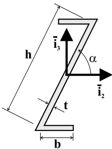
Fig. 8.12. “Z” shaped cross-section.
