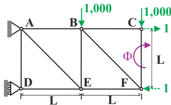
Fig. 9.43. Rotation of a bar in a two-bay planar truss.
