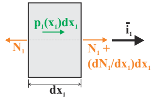
Fig. 6.2. Free body diagram for the axial forces.
