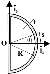
Fig. 8.57. Thin-walled closed semi-circular section.
