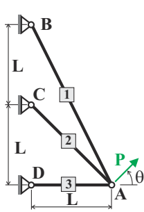
Fig. 10.18. Planar 3-bar truss with load applied at joint A.
