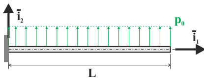
Fig. 15.14. Cantilevered beam with a uniform distributed load.
