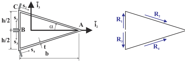
Fig. 8.29. Thin-walled, open triangular section.
