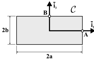
Fig. 12.11. Bar with a rectangular cross-section.
