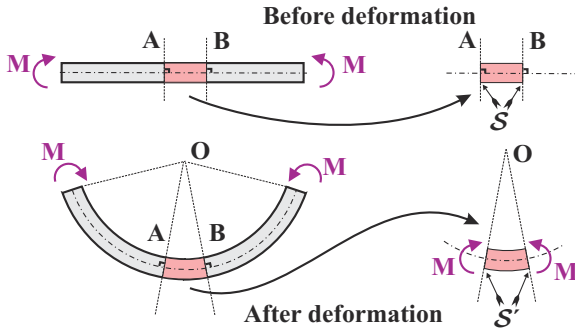
Fig. 5.1. Infinitely long beam under end bending moments.
