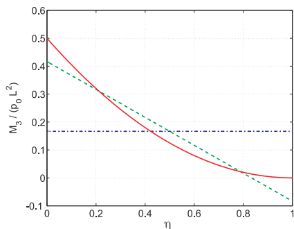
Fig. 11.4. Non-dimensional bending moment for the cantilevered beam. Solid line: three-term polynomial solution (exact solution); dashed line: two-term approximation; dash-dotted line: single-term approximation.
