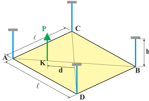
Fig. 4.10. Rigid square plate supported by four elastic cables.
