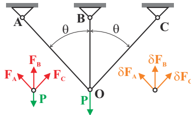
Fig. 10.30. Three-bar truss with applied load (fig. 9.36).
