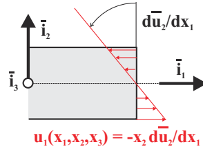
Fig. 5.15. Axial displacement distribution on cross-section.
