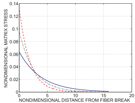
Fig. 2.16. Distribution of matrix shear stress near a fiber break for three material systems.
