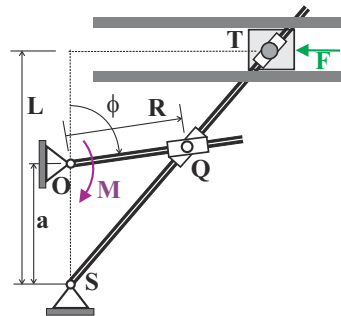
Fig. 9.20. Quick-release mechanism.
