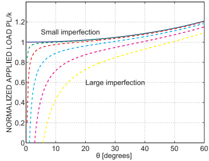
Fig. 14.4. System nonlinear response with various levels of imperfection.
