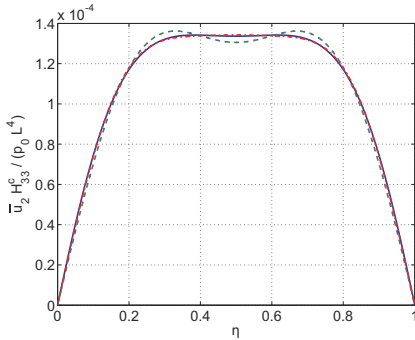
Fig. 11.33. Transverse displacement \bar{u}_2 H_{33}^c / (p_0 L^4) for the exact and approximate solutions versus non-dimensional span. Exact solution: solid line; approximate solution case 1 : dashed line, case 2 : dash-dotted line.
