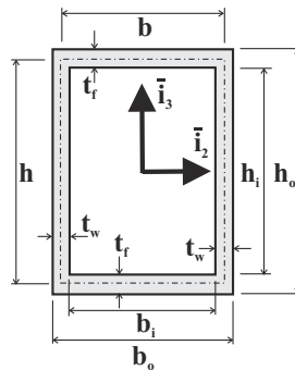
Fig. 6.10. Thin-walled rectangular section.
