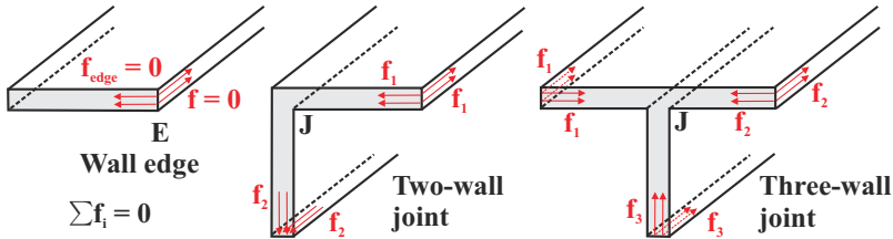
Fig. 8.26. Equilibrium condition at the junction of two or more thin walls.
