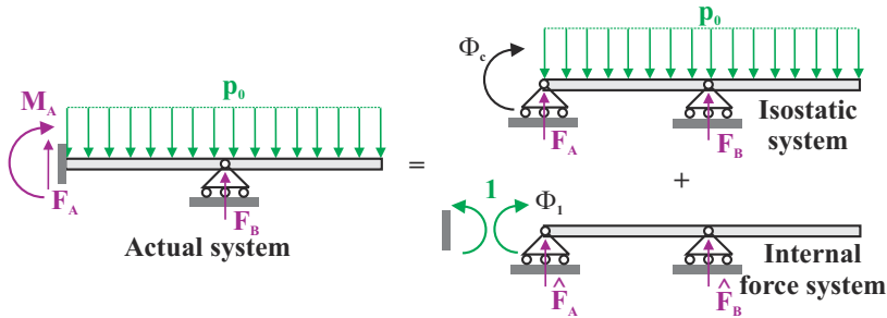
Fig. 9.71. Cantilever with a mid-span support. The isostatic system is obtained by eliminating the mid-span support.
