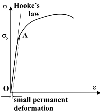
Fig. 2.8. Stress-strain diagram for a ductile material such as aluminum.
