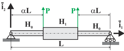
Fig. 5.39. Simply supported beam with varying bending stiffness.
