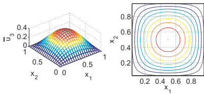
Fig. 16.23. Distribution of transverse displacement, \bar{u}_3 , over the plate.
