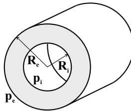
Fig. 3.7. Thick-walled tube subjected to internal and external pressures.
