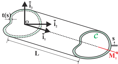
Fig. 9.56. Twisting of a thin walled tube of arbitrary cross-sectional shape.
