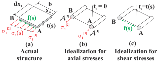
Fig. 8.80. (a): a portion of an actual cross-section; (b): idealization for axial stresses; (c): idealization for shear stresses. (b) and (c) are the sheet-stringer idealization of the actual structure represented in (a).
