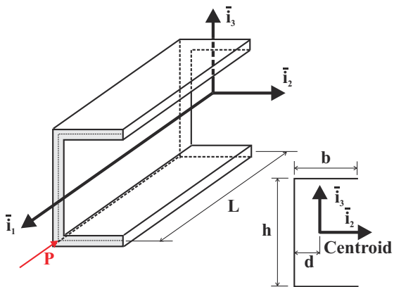
Fig. 14.25. Cantilevered beam with a C-channel cross-section.
