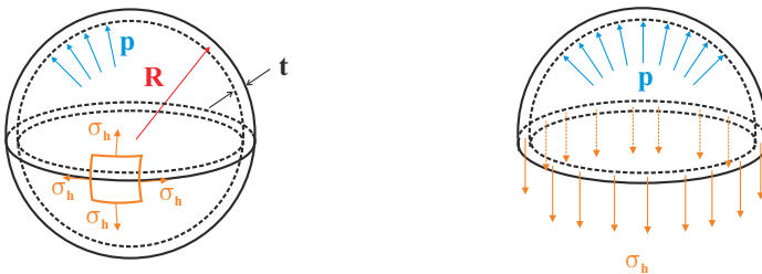
Fig. 4.18. Thin sphere under internal pressure.
