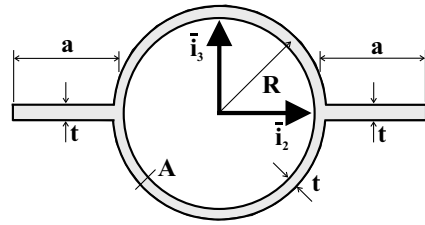
Fig. 8.43. Thin-walled, circular cross-section with flanges.
