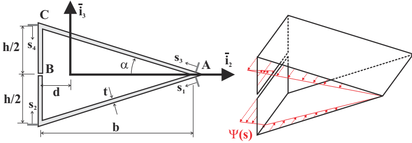
Fig. 8.72. Warping function for a open triangular section.
