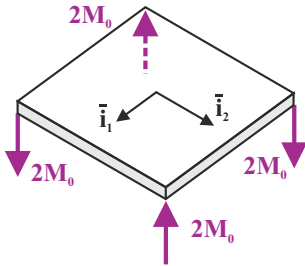
Fig. 16.15. Transverse displacement distribution for corner force bending.
