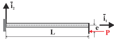
Fig. 14.19. Cantilevered beam subjected to tip axial load with an off-set.
