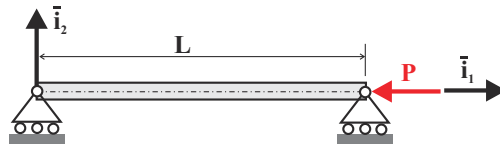
Fig. 14.5. Simply-supported beam with end compressive load.
