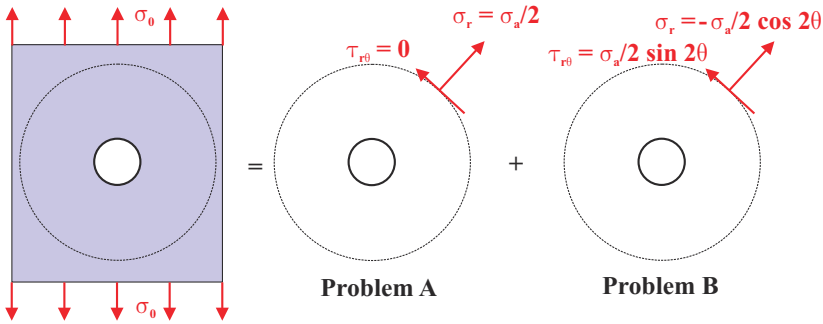
Fig. 3.13. The solution of the desired problem is found by superposing the solutions of two simpler problems: an axisymmetric problem, denoted “problem A” and a non-axisymmetric problem, denoted “problem B”.
