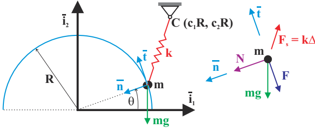
Fig. 9.6. Particle constrained to slide with friction on a circular track.
