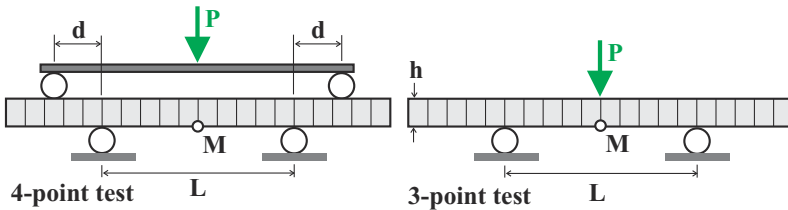
Fig. 15.16. Beam under 4-point and 3-point loading.
