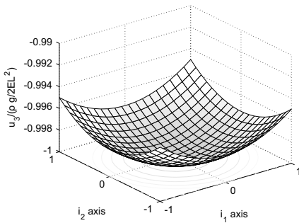
Fig. 3.3. Vertical displacement component, u_3 , of lower surface of the prismatic bar.
