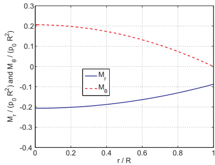
Fig. 16.32. Radial distribution of the non-dimensional bending moments, M_r/(p_0 R^2) and M_\theta/(p_0 R^2) .
