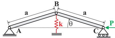
Fig. 9.26. Axially loaded articulated bars with lateral spring restraint.
