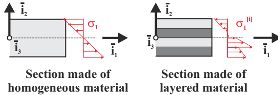
Fig. 5.20. Axial stress distributions in homogeneous and layered sections.
