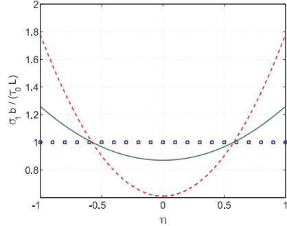
Fig. 12.10. Distribution of axial stress across the panel width at the root of the panel. The uniform distribution predicted by beam theory is indicated by the square boxes. Isotropic material: solid line; anisotropic material: dashed line.
