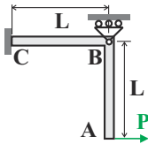
Fig. 9.76. Planar right angle frame with tip load.
