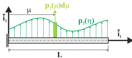
Fig. 5.27. Cantilevered beam under transverse loading.
