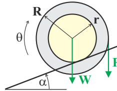
Fig. 9.18. Double-radius wheel on incline.
