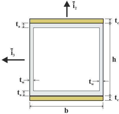
Fig. 5.12. Cross-section of a reinforced rectangular box beam.
