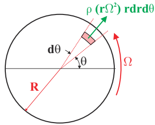
Fig. 3.11. Turbine disk rotating at high angular velocity \Omega .
