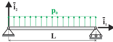
Fig. 11.24. Simply supported beam under a uniform transverse load.
