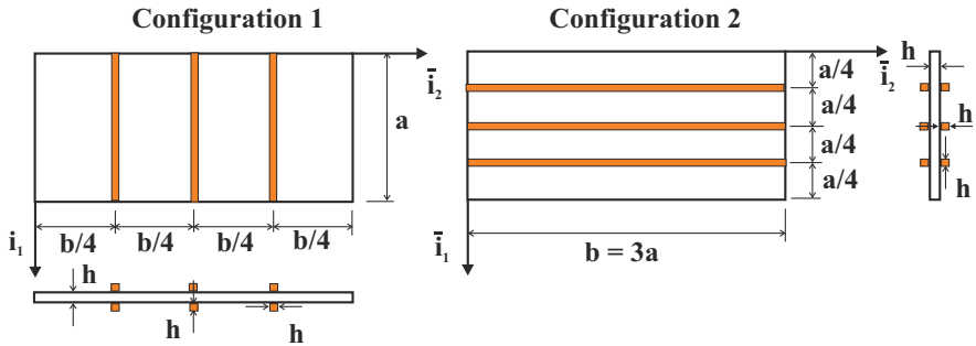
Fig. 16.47. Simply supported rectangular plate with three stiffeners.
