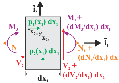
Fig. 5.47. Axial forces acting on an infinitesimal slice of the beam.
