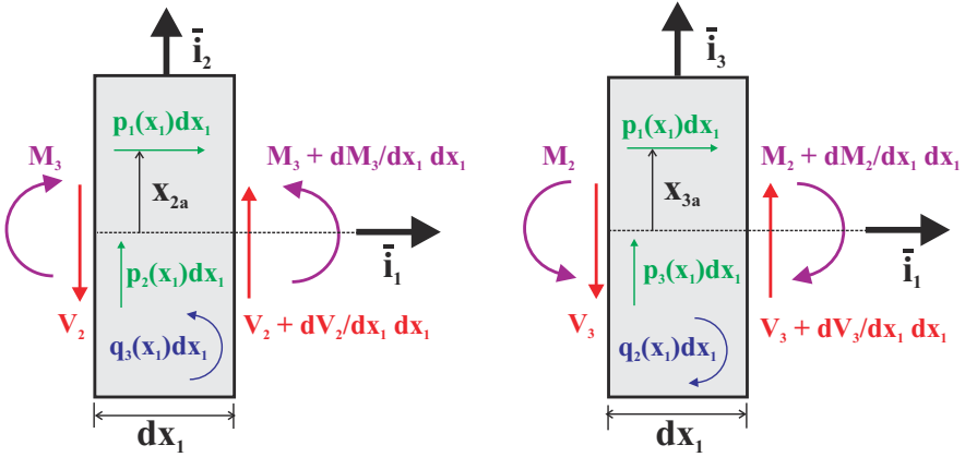
Fig. 6.3. Free body diagram for the transverse shear forces and bending moments. Left figure: view of the (\bar{v}_1, \bar{v}_2) plane; right figure: view of the (\bar{v}_1, \bar{v}_3) plane;
