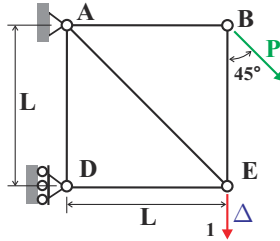
Fig. 13.19. Planar 1-bay truss with thermal loading.
