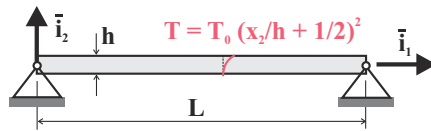
Fig. 14.26. Simply-supported beam under thermal loading.
