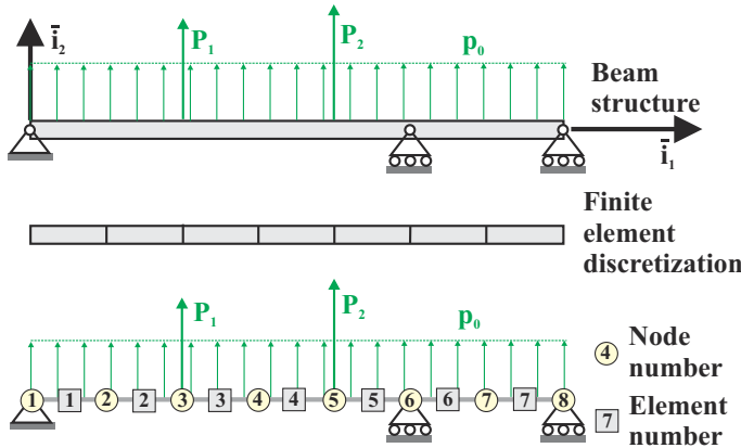
Fig. 11.43. Discretization of a beam into finite elements connected together at nodes.
