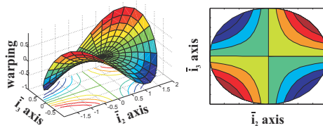
Fig. 7.19. Warping distribution for an elliptic cross-section.
