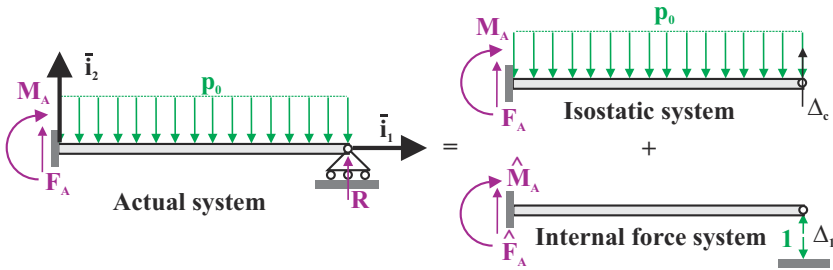
Fig. 9.72. Cantilever with a redundant support.
