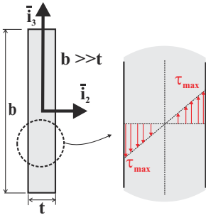
Fig. 7.28. Thin rectangular strip under torsion.
