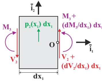
Fig. 5.16. Equilibrium of an infinitesimal slice of the beam.
