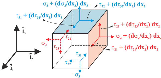
Fig. 1.4. Stress components acting on a differential element of volume. For clarity of the figure, the stress components acting on the faces normal to \bar{i}_1 are not shown.
