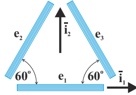
Fig. 1.25. Three strain gauges forming a rosette at the surface of a solid.
