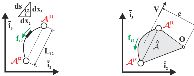
Fig. 8.82. Shear flow in curved sheet.
