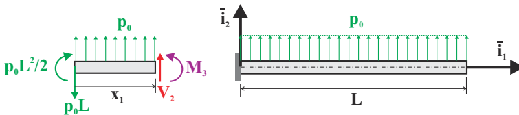
Fig. 5.25. Cantilevered beam under a uniform load.
