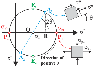
Fig. 1.15. Mohr's circle for visualizing plane stress state.
