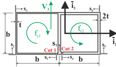
Fig. 8.40. A thin-walled double-box section.
