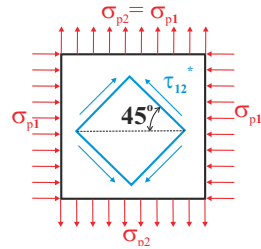
Fig. 1.13. A differential plane stress element in pure shear.
