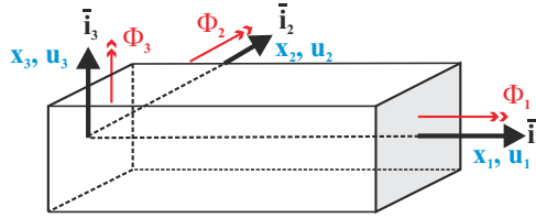
Fig. 5.3. Sign convention for the displacements and rotations of a beam.
