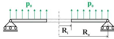
Fig. 16.37. Simply supported annular plate under uniform pressure.
