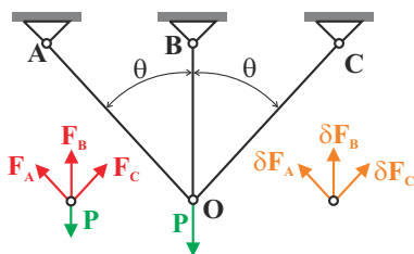
Fig. 9.36. Three-bar truss with applied load.
