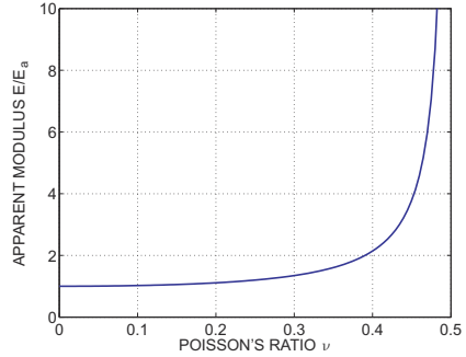
Fig. 2.3. Normalized apparent modulus of elasticity versus Poisson’s ratio.
