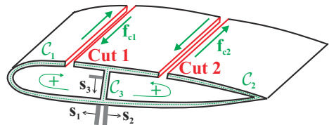
Fig. 8.39. A thin-walled, multi-cellular section.
