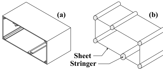
Fig. 8.79. (a) actual cross-section of a thin-walled beam. (b) Sheet-stringer idealization of the same section.
