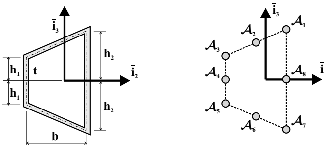
Fig. 6.14. Trapezoidal thin-walled section and lumped representation.
