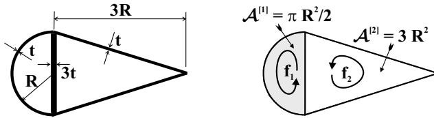
Fig. 8.56. A two-cell thin-walled section under torsion.
