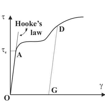
Fig. 2.6. Shear stress-shear strain diagram for a ductile material.
