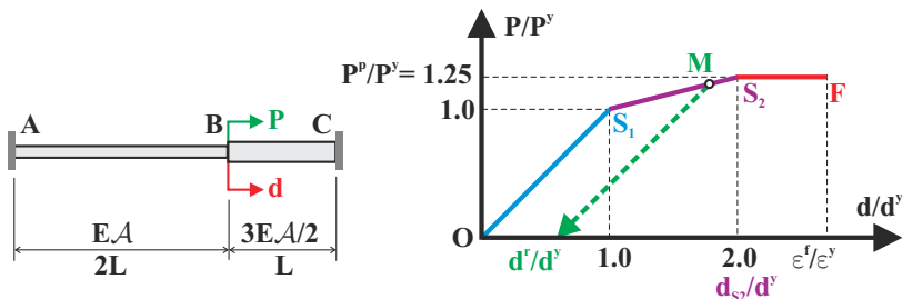
Fig. 13.4. Load-displacement diagram for a two-bar hyperstatic structure with yield stress \sigma_y .
