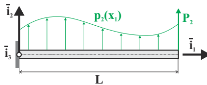
Fig. 11.23. Beam subjected to transverse loads.
