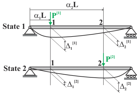
Fig. 10.54. Simply supported beam under two loading states.
