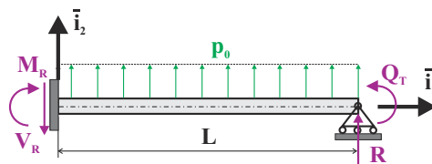
Fig. 11.29. Cantilevered beam with a tip support.
