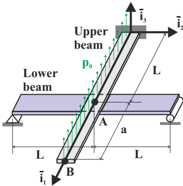
Fig. 5.41. Two beam assembly under transverse load.
