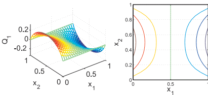
Fig. 16.27. Distribution of transverse shear force, Q_1 , over the plate.
