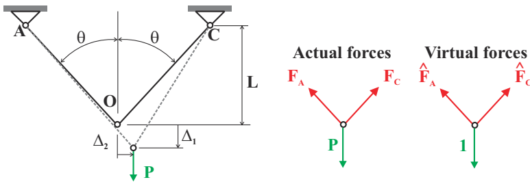
Fig. 9.41. Two-bar truss with unsymmetric properties and vertical load at joint.
