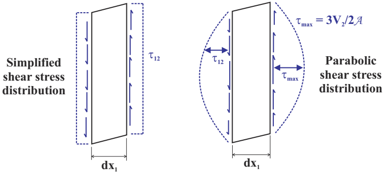
Fig. 15.3. Shear stress distribution for a rectangular section.
