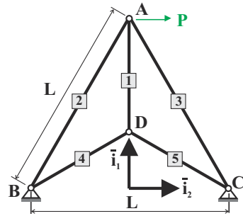
Fig. 10.19. Hyperstatic planar triangular truss.
