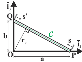
Fig. 8.8. Thin wall component.
