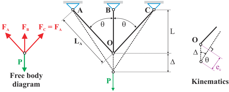
Fig. 4.5. Three bar truss.
