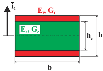
Fig. 15.6. Cross-section made of two materials.
