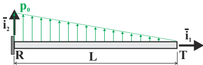
Fig. 10.50. Cantilevered beam subjected to half-span loading.
