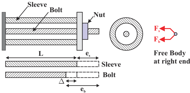
Fig. 4.15. Prestressed bolt-sleeve assembly.
