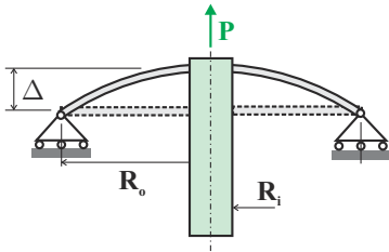
Fig. 16.36. Simply supported circular plate with center rigid shaft.
