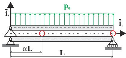
Fig. 5.45. Superposed simply supported beams.
