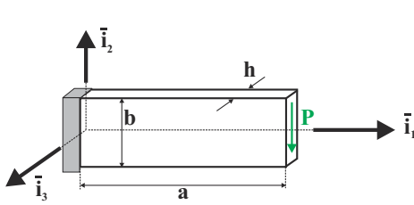
Fig. 16.58. Cantilevered plate under tip shear load.
