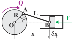
Fig. 9.12. The crank-slider mechanism.
