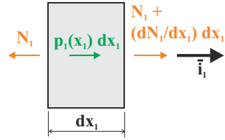
Fig. 5.8. Axial forces acting on an infinitesimal slice of the beam.
