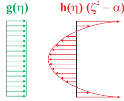
Fig. 12.8. The distribution of axial displacement.
