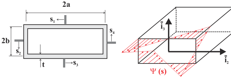
Fig. 8.74. Thin-walled beam with a rectangular cross-section.
