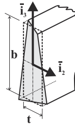
Fig. 7.29. Warping function for a thin rectangular strip.
