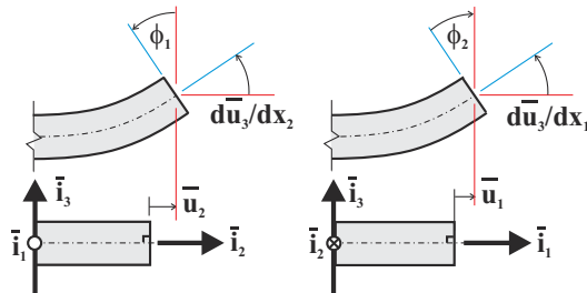
Fig. 16.2. Rotations of the normal line and slopes of the plate.
