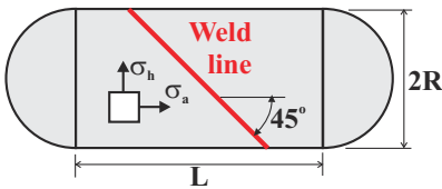
Fig. 1.19. Pressure vessel with a weld line.
