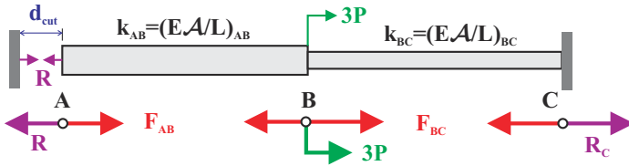
Fig. 4.4. Two bars connected in series with ends fixed and a cut at point A .
