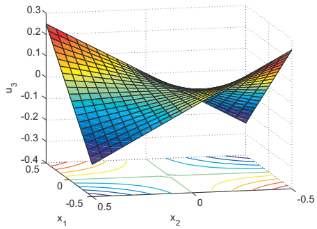
Fig. 16.16. Transverse displacement distribution for corner force bending.
