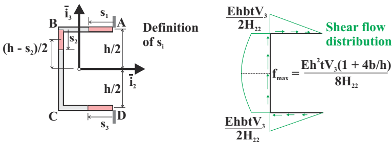
Fig. 8.25. Distribution of shear flow over the C-channel cross-section.
