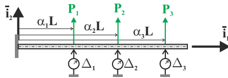
Fig. 5.28. Cantilevered wing under three concentrated loads.
