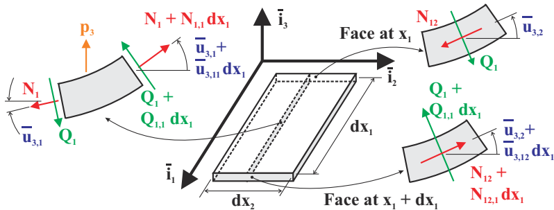
Fig. 16.49. Free body diagram of a deformed differential element of the plate.
