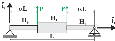
Fig. 11.39. Simply supported beam with variable bending stiffness.
