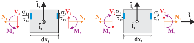
Fig. 5.5. Sign convention for the sectional stress resultants.
