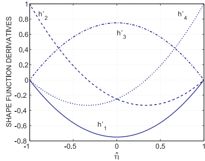
Fig. 11.46. Derivatives of the beam element shape functions. h'_1 : solid line; h'_2 : dashed line; h'_3 : dash-dotted line; h'_4 : dotted line.
