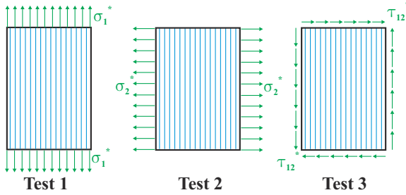
Fig. 2.26. Three tests for the determination of the strength of a lamina
