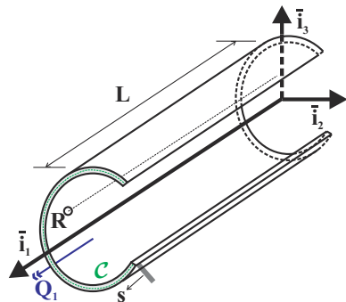
Fig. 8.70. Thin-walled beam subjected to an applied torque.
