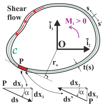
Fig. 8.9. Sign conventions for the shear flow, f(s) .
