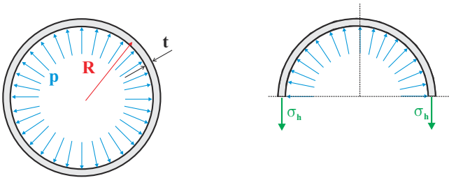
Fig. 4.16. Thin ring under internal pressure.
