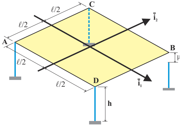
Fig. 4.14. A rigid plate supported by four identical elastic bars with a manufacturing imperfection.
