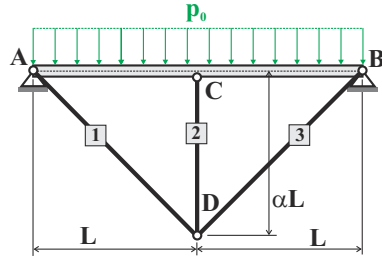
Fig. 10.37. Simply supported beam with uniform load and truss bracing.
