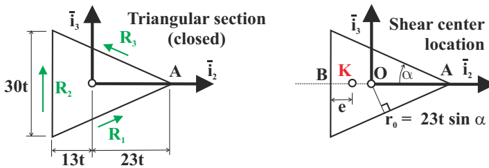
Fig. 8.47. Shear center for thin-walled triangular section.
