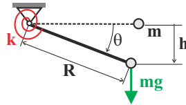
Fig. 10.11. Torsional spring supporting a weight.
