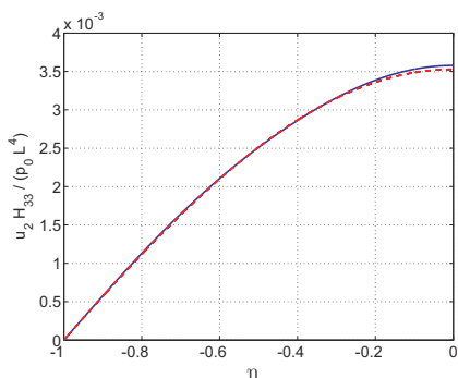
Fig. 11.13. Transverse displacement over left half-span of beam under uniform load for \bar{k} = 10^2 . Solid line: exact solution; dashed line: three-term approximate solution.
