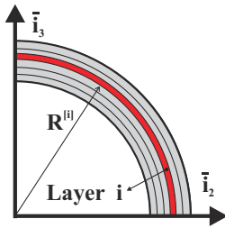
Fig. 7.7. Thin-walled tube made of layered materials.
