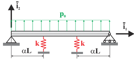
Fig. 11.36. Simply supported beam with two mid-span springs.
