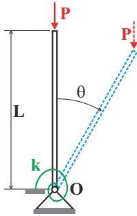
Fig. 14.1. Bar with a root torsional spring.
