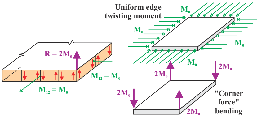
Fig. 16.10. Loading the edge of a plate with a uniform twisting moment. Plate under corner force bending
