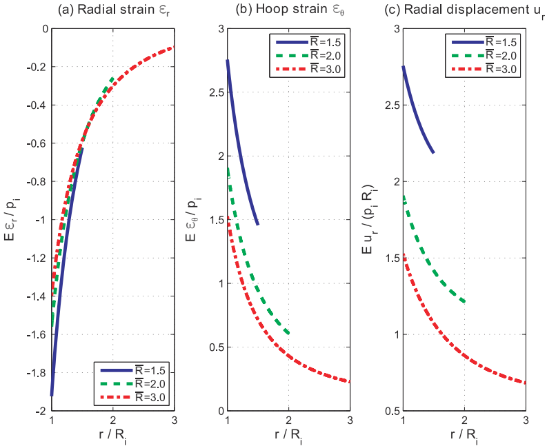
Fig. 3.9. Plots of the non-dimensional radial strain, E\epsilon_r/p_i , hoop strain E\epsilon_\theta/p_i , and radial displacement, E u_r/(R_i p_i) , for three different thickness ratios \bar{R} = 1.5, 2.0, 3.0 .
