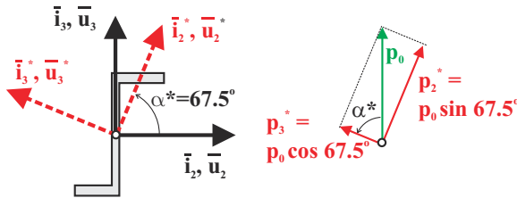
Fig. 6.19. The principal axes of bending for the thin walled section.
