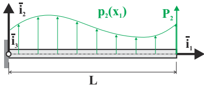
Fig. 5.14. Beam subjected to transverse loads.
