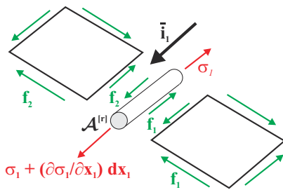
Fig. 8.81. Axial equilibrium of stringer with two joining sheets.
