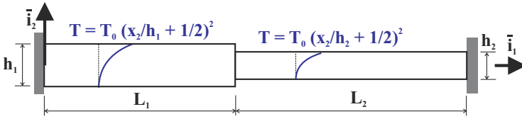
Fig. 13.23. Clamped-clamped beam subjected to parabolic thermal gradients.
