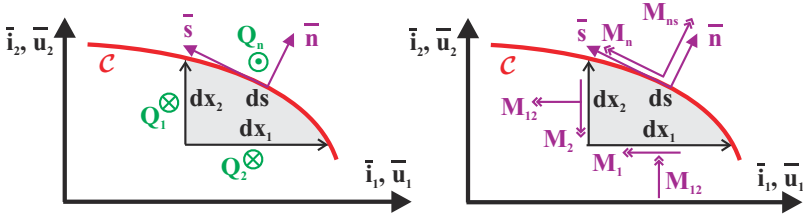
Fig. 16.43. The global coordinate system and the local coordinate system along the edge of the plate.
