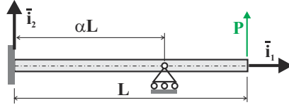
Fig. 15.11. Cantilevered beam with intermediate support.
