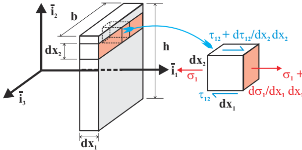
Fig. 15.2. Configuration of a differential element of the beam.
