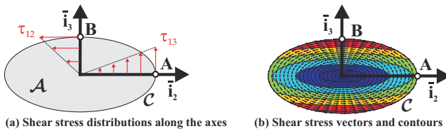
Fig. 7.18. Shear stress distribution for an elliptical cross-section.
