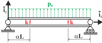
Fig. 5.43. Simply supported beam connected by spring.
