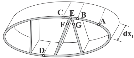
Fig. 8.53. A thin-walled, multi-cellular section under torsion.
