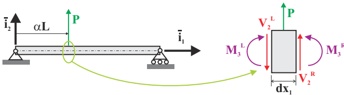
Fig. 5.23. Simply supported beam with one concentrated load.
