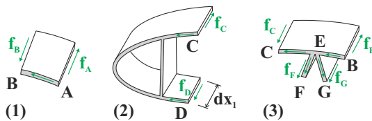
Fig. 8.54. Free-body diagrams of the thin-walled, multi-cellular section.
