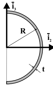
Fig. 7.33. Semi-circular open cross-section.
