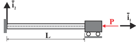
Fig. 14.23. Clamped-clamped beam under tip load.
