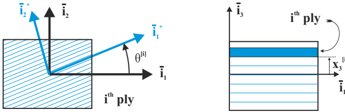
Fig. 16.19. Definition of a laminated plate.
