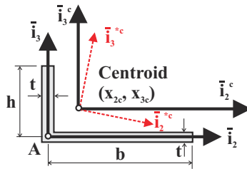
Fig. 6.15. Thin-walled, L shaped cross-section.
