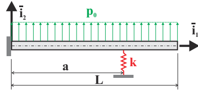
Fig. 5.42. Cantilevered beam with concentrated spring.
