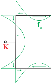
Fig. 8.75. Shearing flow, f_w , for a C-channel.
