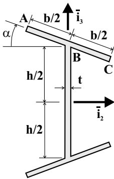
Fig. 8.18. Skewed “T” shaped cross-section.
