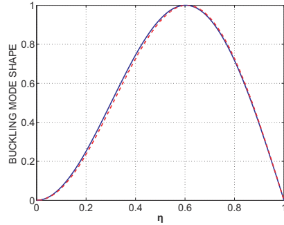
Fig. 14.13. Buckling mode shape for the cantilevered beam with tip support. Exact solution: solid line; approximate solution ( n = 1 ): dashed line.
