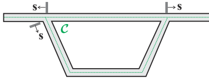
Fig. 8.3. Thin-walled beam with open and closed components.
