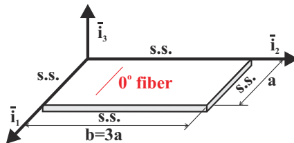
Fig. 16.60. Simply-supported rectangular plate
