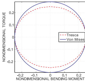
Fig. 7.11. Yield envelopes predicted by Tresca's and von Mises' criteria plotted in the non-dimensional loading space.
