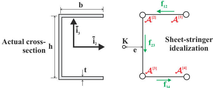
Fig. 8.83. Sheet-stringer model for C-channel section.
