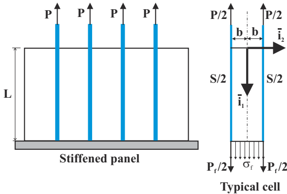
Fig. 12.18. Configuration of the stiffened panel.
