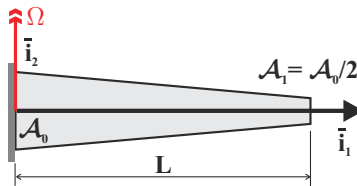
Fig. 5.11. A helicopter blade rotating at an angular speed \Omega .
