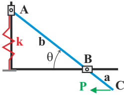
Fig. 9.23. Lever with sliding pivots and spring.
