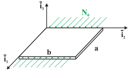
Fig. 16.59. Simply supported plate on an elastic foundation.
