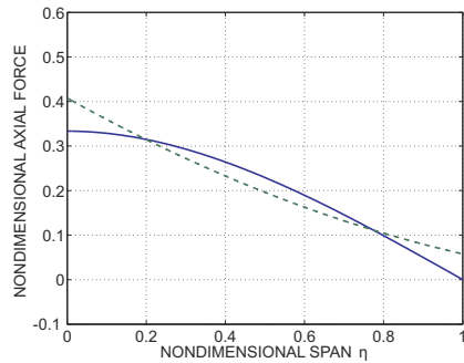
Fig. 11.20. Non-dimensional axial force, N_1 / (\rho A_0 \Omega^2 L^2) , versus \eta . Strong statement of equilibrium: solid line; weak statement: dashed line.
