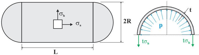
Fig. 4.17. Pressure vessel under internal pressure.
