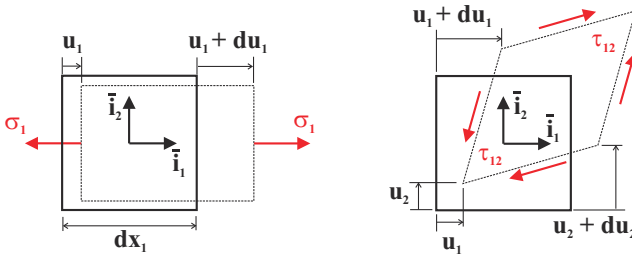
Fig. 9.50. Deformation of a differential element of a solid.
