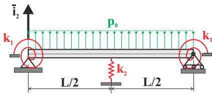
Fig. 11.37. Simply supported beam with mid-span and end point springs.
