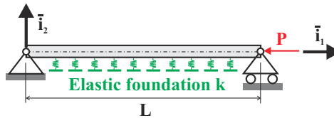
Fig. 15.19. Simply supported beam on an elastic foundation.
