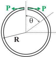
Fig. 10.42. Ring subjected to internal forces acting in the plane of the ring.
