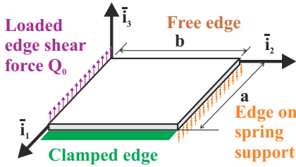
Fig. 16.17. Rectangular plate with various boundary conditions.
