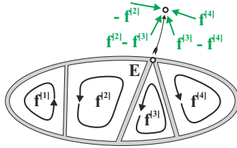
Fig. 8.55. Shear flows in each cell of a thin-walled, multi-cellular section.
