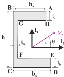
Fig. 6.22. “C” shaped cross-section.
