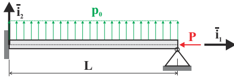
Fig. 14.20. Cantilevered beam with tip support subjected to a compressive load.
