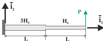
Fig. 11.35. Cantilevered beam with nonuniform bending stiffness.
