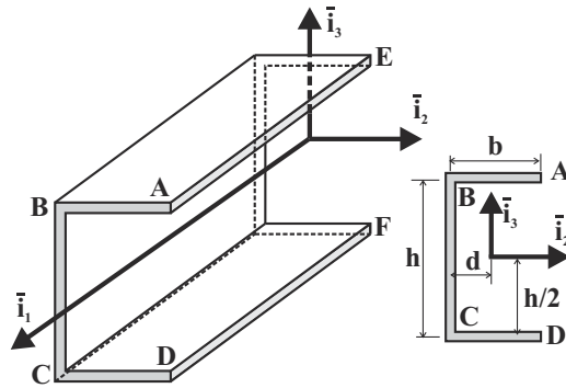
Fig. 8.24. Cantilevered beam with a C-channel cross-section.
