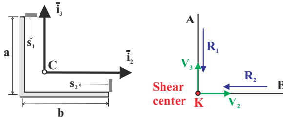
Fig. 8.33. Shear center in thin-walled right-angle section
