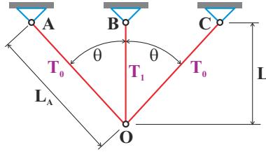
Fig. 4.13. Three bar truss subjected to temperature differentials.
