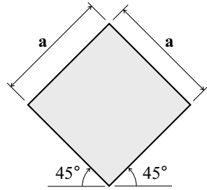
Fig. 13.11. Beam diamond cross-section.
