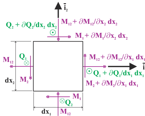
Fig. 16.5. Free body diagram for the equilibrium of bending moment and shear forces.
