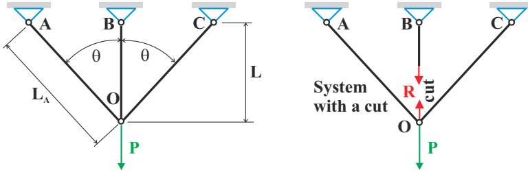
Fig. 4.7. Three bar truss.
