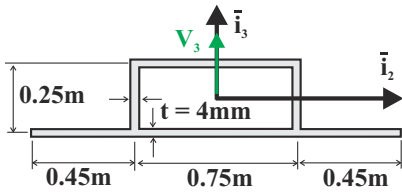
Fig. 8.44. High lift device subjected to a transverse shear force.
