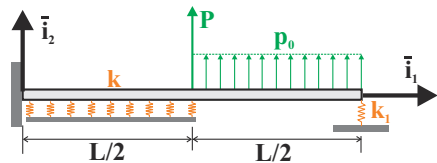
Fig. 12.13. Simply supported beam with partial elastic foundation.
