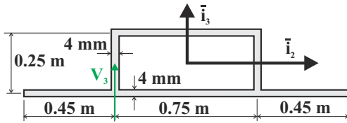
Fig. 8.59. High lift device subjected to a transverse shear force.
