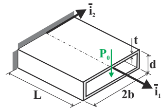
Fig. 12.6. Box beam subjected to tip load.
