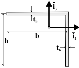
Fig. 8.14. “L” shaped cross-section.
