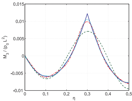
Fig. 11.31. Bending moment M_3/(p_0L^2) for the exact and approximate solutions versus non-dimensional span. Exact solution: solid line; approximate solution case 1: dashed line, case 2: dash-dotted line, case 3: dotted line.
