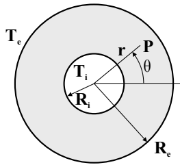
Fig. 13.15. Thick tube in plane strain state subjected to a temperature field.
