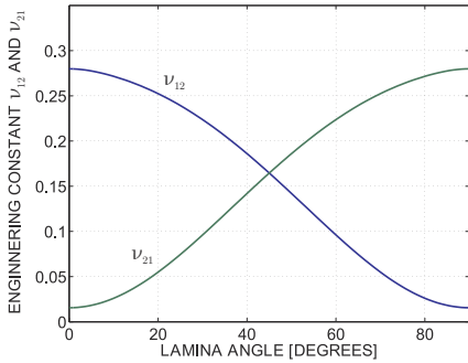
Fig. 2.24. Variation of engineering constants \nu_{12} and \nu_{21} with lamina angle \theta .
