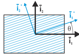
Fig. 2.18. Definition of two axis systems for a lamina.
