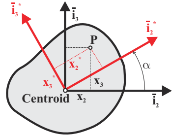
Fig. 6.4. Rotation of the axes of the cross-section.
