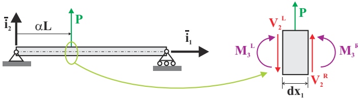
Fig. 11.25. Simply supported beam with one concentrated load.
