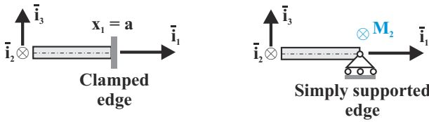
Fig. 16.6. Boundary conditions for clamped and simply supported edges.
