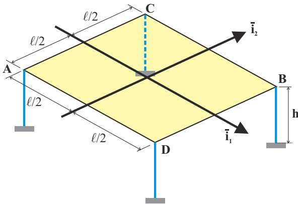
Fig. 13.20. A rigid plate supported by four identical elastic bars.
