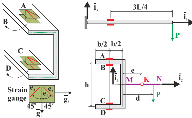
Fig. 8.49. Cantilever beam with C-section under offset tip load.
