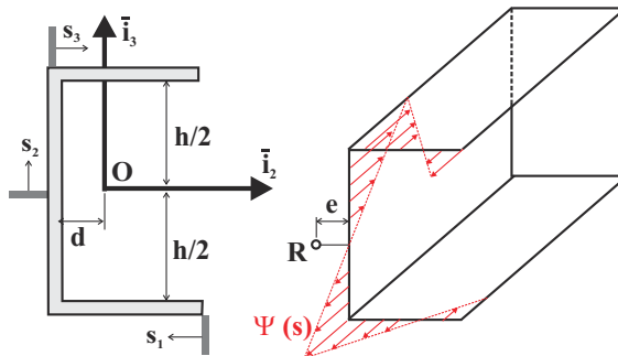
Fig. 8.71. The warping function for a C-channel.
