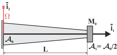
Fig. 11.21. A helicopter blade with a tip mass rotating at an angular speed \Omega .
