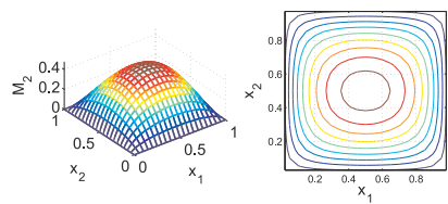
Fig. 16.26. Distribution of bending moment, M_2 , over the plate.
