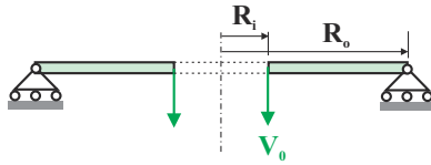
Fig. 16.33. Diametric cross-section through a simply supported annular plate subjected to a uniform shear force around its inner edge.
