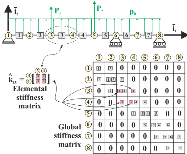
Fig. 11.47. Illustration of the assembly procedure.
