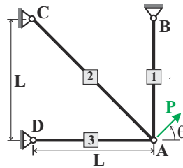
Fig. 10.21. Planar rectangular 3-bar truss with unequal axial stiffnesses.
