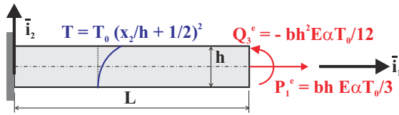
Fig. 13.21. Cantilevered beam under parabolic thermal gradient.
