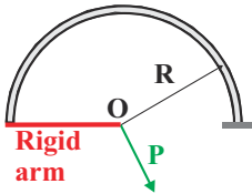
Fig. 10.52. Semi-circular beam with a rigid arm.
