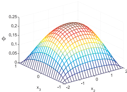
Fig. 7.22. Stress function, \phi .
