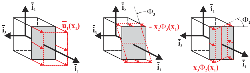
Fig. 5.2. Decomposition of the axial displacement field.
