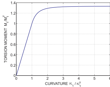
Fig. 13.14. The moment-curvature diagram for a section made of elastic-perfectly plastic material.
