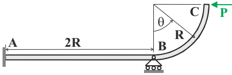
Fig. 9.80. Curved cantilevered beam with tip load.
