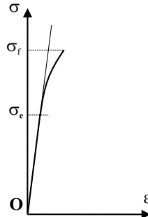
Fig. 2.9. Stress-strain diagram for a brittle material.
