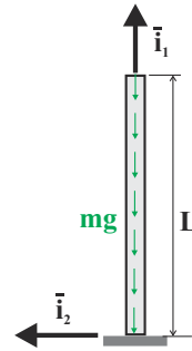
Fig. 14.21. Flag pole standing under its own weight.
