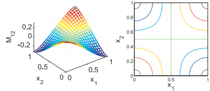
Fig. 16.24. Distribution of twisting moment, M_{12} , over the plate.
