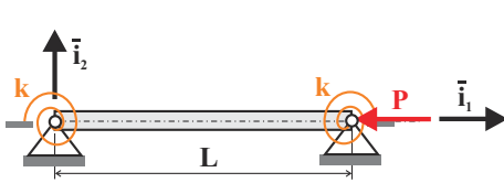
Fig. 14.16. Simply-supported beam with end torsional springs.
