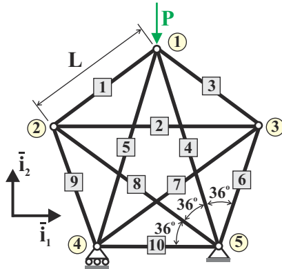
Fig. 10.26. Pentagonal truss with nodes and members defined for analysis using finite element approach.
