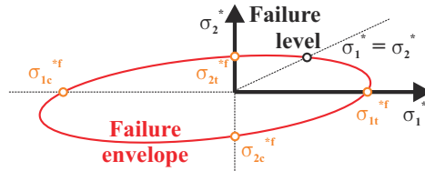
Fig. 2.27. Stress space for a lamina in biaxial stress state.
