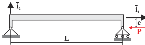
Fig. 14.8. Pinned-pinned beam with eccentric end loads.
