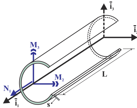
Fig. 8.11. Thin-walled beam subjected to axial forces and bending moments.
