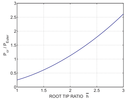
Fig. 14.15. Buckling load for tapered cantilevered beam as a function of the root depth to the tip depth, \bar{h} .
