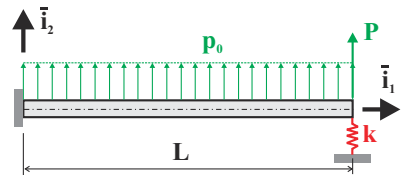
Fig. 5.38. Cantilevered beam with tip spring.
