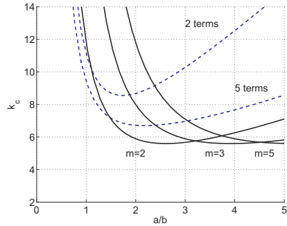
Fig. 16.57. Buckling parameter, k_c , versus plate aspect ratio.
