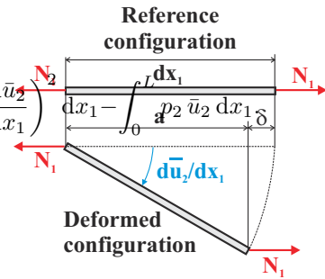
Fig. 14.11. A differential element of the beam in the deformed configuration.
