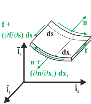
Fig. 8.10. Equilibrium of a differential element of the wall.
