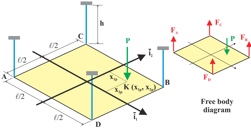
Fig. 4.6. A rigid plate supported by four identical elastic cables.
