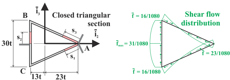
Fig. 8.37. Non-dimensional shear flow distribution in a closed triangular section.
