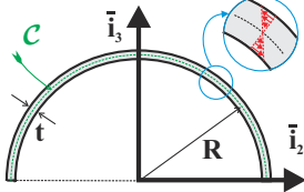
Fig. 7.30. Semi-circular thin-walled open section.
