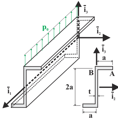
Fig. 9.55. Cantilevered Z-section beam under a uniform load.
