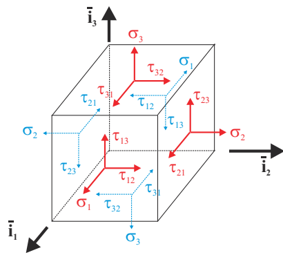
Fig. 1.3. Sign conventions for the stress components acting on a differential volume element. All stress components shown here are positive.
