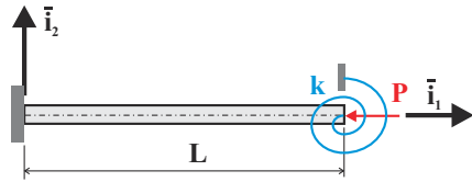
Fig. 15.17. Cantilevered beam with tip torsional spring.
