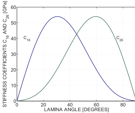
Fig. 2.21. Variation of the coupling stiffness coefficients, C_{16} and C_{26} , with the lamina angle \theta .
