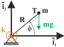
Fig. 9.13. Pendulum with torsional spring.
