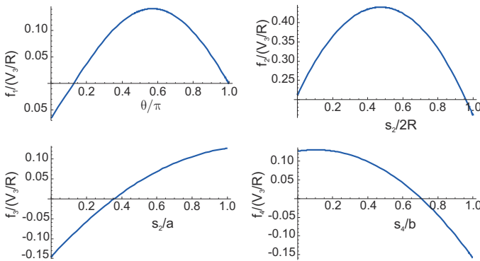
Fig. 8.68. Shear flow distribution in each segment of the 2-cell wing cross-section.
