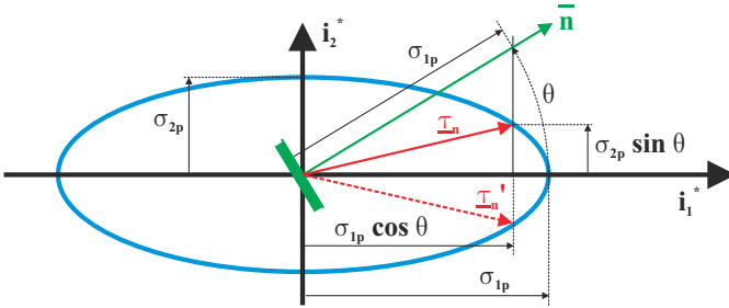
Fig. 1.17. Lamé's ellipse. Stress vector \underline{\tau}_n corresponds to positive principal stresses whereas stress vector \underline{\tau}'_n corresponds to \sigma_{p1} > 0 and \sigma_{p2} < 0 .
