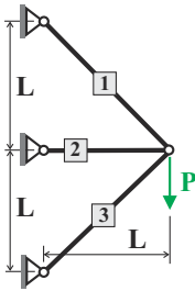
Fig. 10.36. 3-bar truss with unequal bar stiffness properties.
