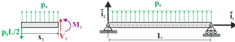
Fig. 5.22. Simply supported beam under a uniform transverse load.
