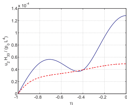
Fig. 11.14. Transverse displacement over left half-span of beam under uniform load for \bar{k} = 10^4 . Solid line: exact solution; dashed line: three-term approximate solution.
