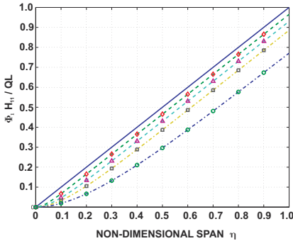
Fig. 8.76. Twist distribution for the closed rectangular section under non-uniform torsion. \bar{k} = 16.54 ( \diamond ), \bar{k} = 8.27 ( \triangle ), \bar{k} = 5.04 ( \square ), \bar{k} = 2.52 ( \circ ).
