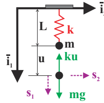
Fig. 9.4. A particle suspended to an elastic spring.
