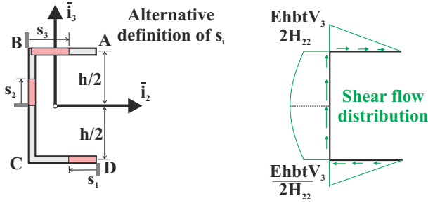
Fig. 8.27. Distribution of shear flow over the C-channel cross-section for an alternative definition of the curvilinear variable.
