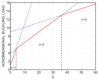
Fig. 14.29. Non-dimensional critical loads P_{cr n}/P_{Euler} for n = 1, 2, and 3 .
