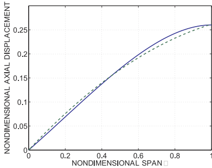
Fig. 11.19. Non-dimensional axial displacement, \bar{u}_1 E / (\rho A_0^2 L^3) , versus \eta . Strong statement of equilibrium: solid line; weak statement: dashed line.
