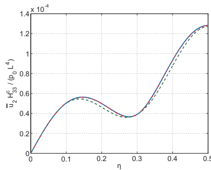
Fig. 11.30. Transverse displacement \bar{u}_2 H_{33}^c / (p_0 L^4) for the exact and approximate solutions versus non-dimensional span. Exact solution: solid line; approximate solution case 1 : dashed line, case 2 : dash-dotted line, case 3 : dotted line.
