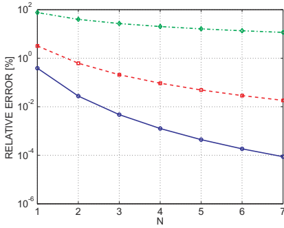
Fig. 11.7. Relative error of the approximate solution compared to the exact solution. Solid line: mid-span transverse displacement (○); dashed line: mid-span bending moment (□); dash-dotted line: root shear force (◇).
