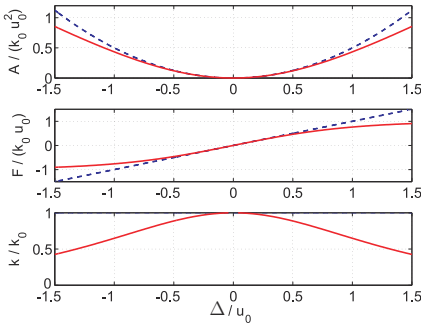
Fig. 10.7. Nonlinear spring with the constitutive law given by eq. (10.24). Top figure: strain energy; middle figure: force; bottom figure: stiffness. Solid line: nonlinear spring; dashed line: linear spring.
