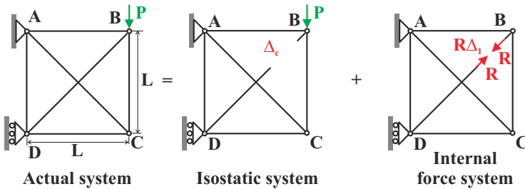
Fig. 9.67. Six-bar hyperstatic truss.
