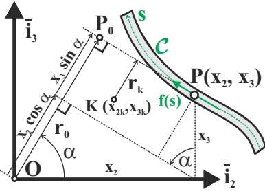
Fig. 8.7. Geometry of a differential element of the wall.
