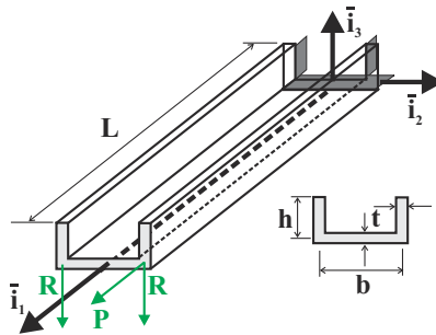
Fig. 6.30. Cantilevered beam with “U” shaped section under tip axial loads.
