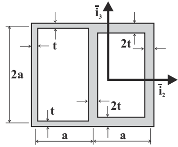
Fig. 8.60. Thin-walled 2-cell rectangular section with variable wall thicknesses.
