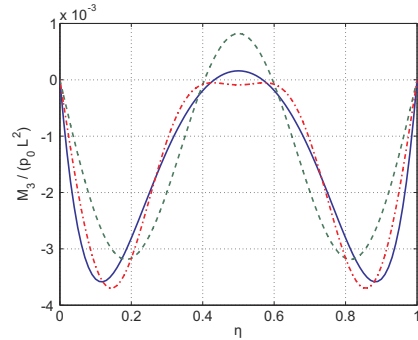
Fig. 11.34. Bending moment M_3 / (p_0 L^2) for the exact and approximate solutions versus non-dimensional span. Exact solution: solid line; approximate solution case 1 : dashed line, case 2 : dash-dotted line.
