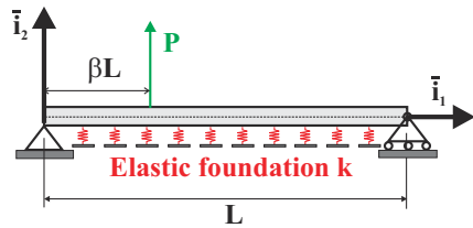
Fig. 11.42. Beam with elastic foundation subjected to a concentrated load.
