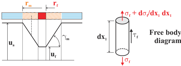
Fig. 2.14. Displacement definition and free body diagram of a differential element of fiber.
