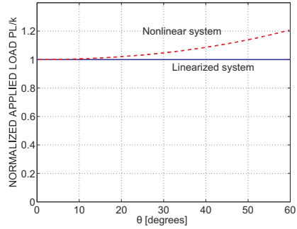
Fig. 14.2. Behavior of a perfect system.
