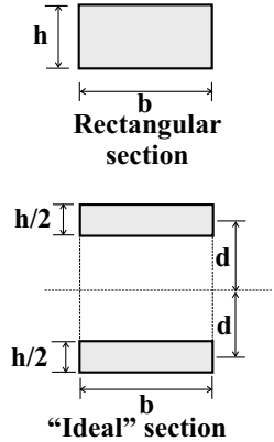
Fig. 5.21. A rectangular section, and the ideal section.
