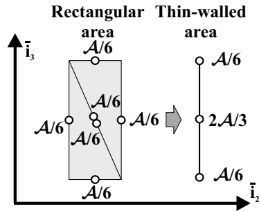
Fig. 6.12. Rectangular area equivalent lumped areas.
