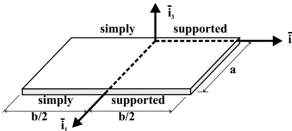
Fig. 16.29. Rectangular plate simply supported along two opposite edges.
