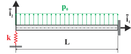
Fig. 5.40. Cantilevered beam under uniform load with a root spring.
