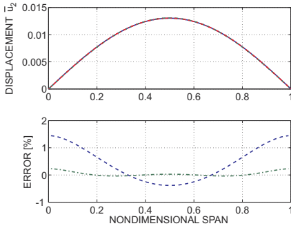
Fig. 11.26. Top figure: transverse displacement \bar{u}_2 ; bottom figure: error. Exact solution: solid line; Approximate solution: dashed line (case 1), dash-dotted line (case 2).
