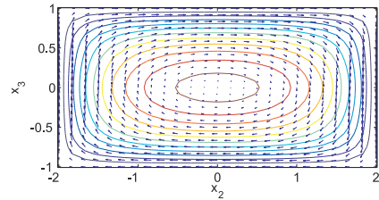
Fig. 7.23. Distribution of shear stress over cross-section. The arrows represent the shear stresses; the contours represent constant values of the stress function \phi .
