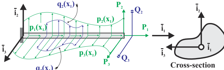
Fig. 6.1. Beam with arbitrary three-dimensional loading.
