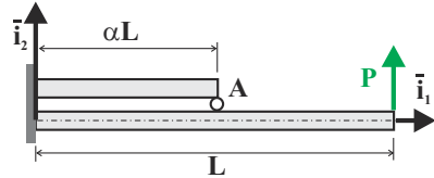
Fig. 5.44. Cantilevered beam with intermediate support.
