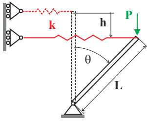
Fig. 10.12. Rigid bar with tip spring under compressive load. Original and deformed configurations.
