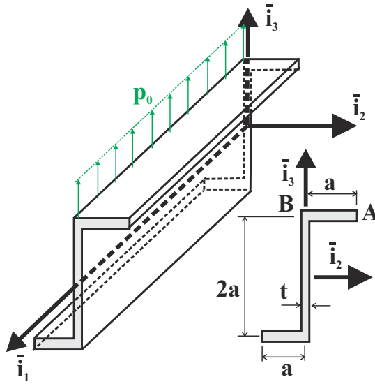
Fig. 6.18. Thin-walled cantilevered beam under a uniform transverse load.
