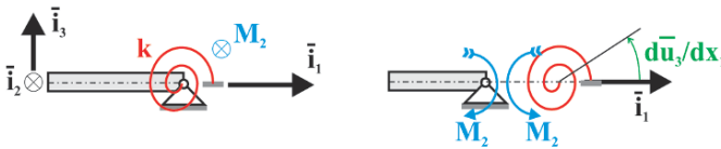
Fig. 16.9. Boundary conditions for an edge with a rotational spring.
