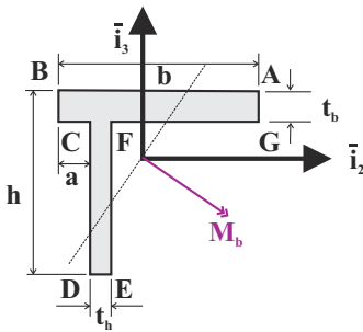
Fig. 6.24. “T” shaped cross-section.
