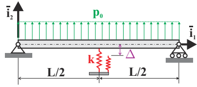
Fig. 5.36. Simply supported beam with mid-span spring featuring a clearance \Delta .
