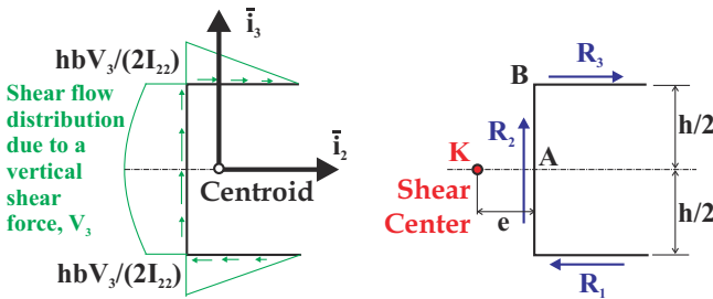
Fig. 8.31. Shear center in C-channel section.
