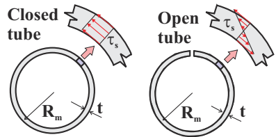
Fig. 8.51. A thin-walled open tube and a thin-walled closed tube.
