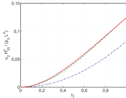
Fig. 11.3. Non-dimensional transverse displacement field for the cantilevered beam. Solid line: three-term polynomial solution (exact solution); dashed line: two-term approximation; dashed-dotted line: single-term approximation.
