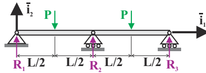
Fig. 10.31. A beam on 3 simple supports.
