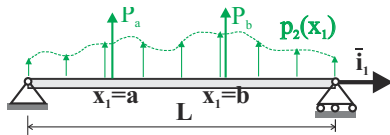
Fig. 11.1. Simply-supported beam subjected to distributed lateral load and.
