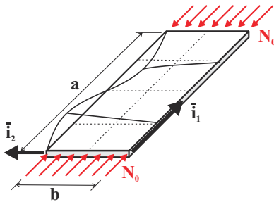
Fig. 16.53. Plate with three edges simply supported and the fourth side edge free.
