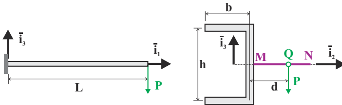
Fig. 8.69. Cantilever beam with C-section under offset tip load.
