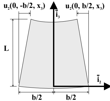
Fig. 3.4. Lateral displacement component, u_2 , of the left and right sides of prismatic bar.
