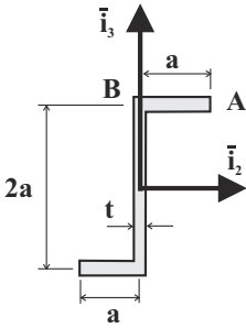
Fig. 6.16. “Z” shaped cross-section of a beam.
