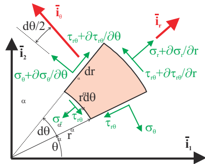
Fig. 3.6. Stresses acting on a differential area defined in polar coordinates.
