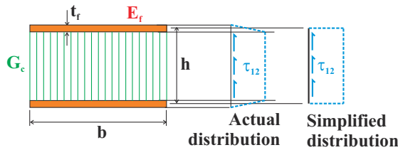
Fig. 15.5. Shear stress distribution on the cross-section of a sandwich section.
