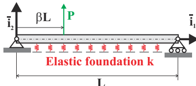
Fig. 5.46. Beam with elastic foundation subjected to a concentrated load.
