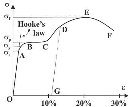
Fig. 2.5. Stress-strain diagram for a ductile material such as mild steel.
