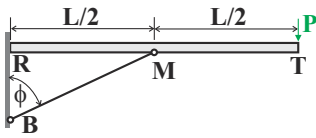
Fig. 9.78. Cantilevered beam with supporting truss.
