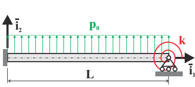
Fig. 5.35. Cantilevered beam with tip support and torsional spring.
