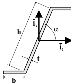
Fig. 8.13. “Z” shaped cross-section.
