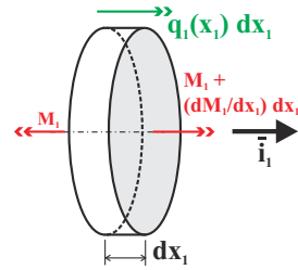
Fig. 7.6. Torsional loads acting on an infinitesimal slice of the bar.
