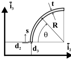
Fig. 8.23. Stiffness static moments for a thin-walled circular arc.
