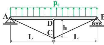
Fig. 9.79. Simply supported beam with supporting truss.
