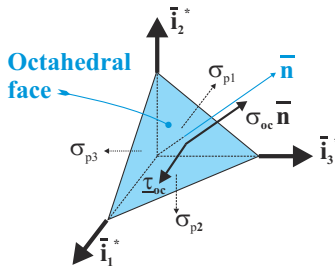
Fig. 1.8. The octahedral face.
