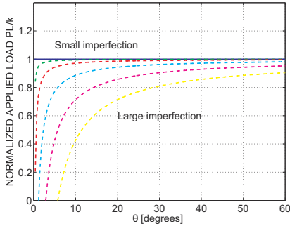
Fig. 14.3. System linearized response with various levels of imperfection.
