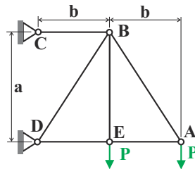
Fig. 9.45. Planar truss with nonlinear material properties.
