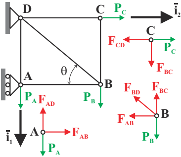
Fig. 9.31. Configuration of the 5-bar truss.
