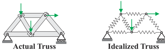
Fig. 9.28. Planar truss and its idealization as an assembly of rectilinear springs.
