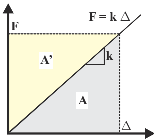
Fig. 10.5. Constitutive law for a linearly elastic spring.
