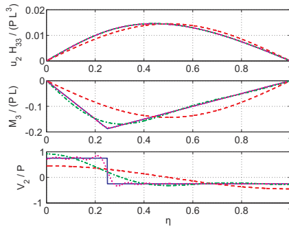
Fig. 11.10. Simply-supported beam subjected to a concentrated transverse load. Top figure: transverse displacement, \bar{u}_2 H_{33}^c / (PL^3) ; middle figure: bending moment, M_3 / (PL) ; lower figure: shear force, V_2 / P . Exact solution: solid line; single term solution: dashed line; three-term solution: dash-dotted line; 24-term solution: dotted line.
