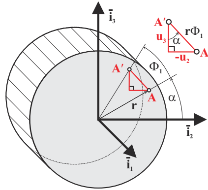
Fig. 7.3. In-plane displacements for a circular cylinder. The cross-section undergoes a rigid body rotation.
