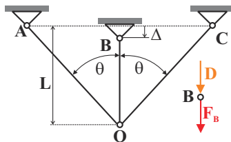
Fig. 10.29. Three-bar truss with prescribed displacement (see fig. 9.37).
