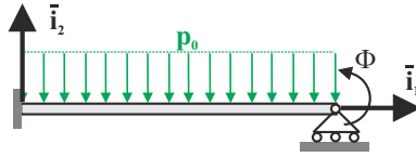
Fig. 9.73. Tip rotation for cantilever with a redundant tip support.
