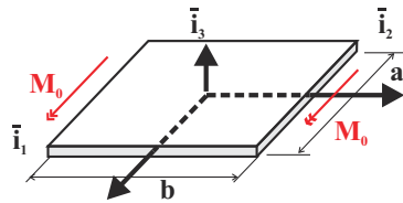
Fig. 16.18. Rectangular plate with edge moments.
