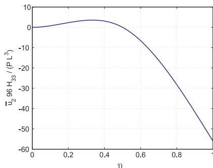
Fig. 11.49. Deflection of beam elements 1 and 2.
