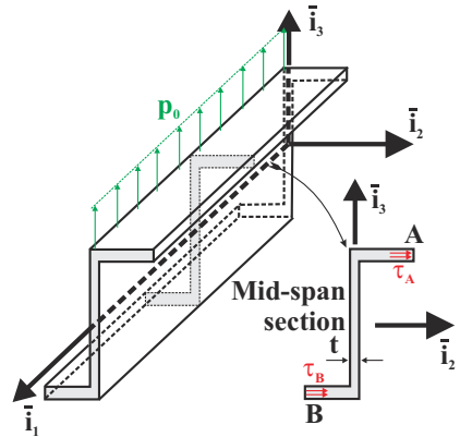
Fig. 1.10. Shear stresses at points A and B on cross-section.
