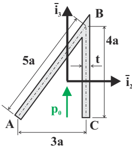
Fig. 6.26. Inverted “V” shaped cross-section.
