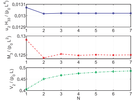
Fig. 11.8. Convergence of approximate solution as a function of the number of degrees of freedom. Solid line: mid-span transverse displacement (○); dashed line: mid-span bending moment (□); dash-dotted line: root shear force (◇).
