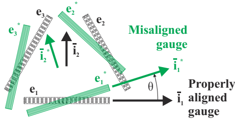
Fig. 1.27. Delta rosette with an angular misalignment of \theta .
