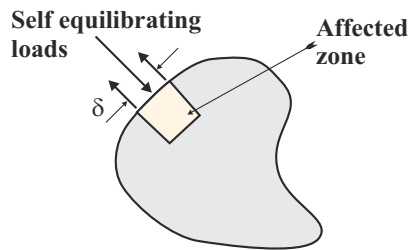
Fig. 4.20. Body subjected to a set of self-equilibrating loads
