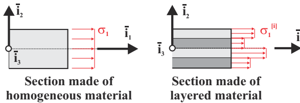
Fig. 5.10. Axial stress distribution for sections made of homogeneous and layered materials.
