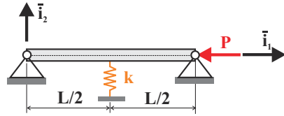
Fig. 14.17. Simply-supported beam with a mid-span spring.
