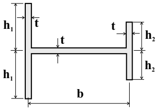
Fig. 7.34. "H" cross-section of a thin-walled beam.
