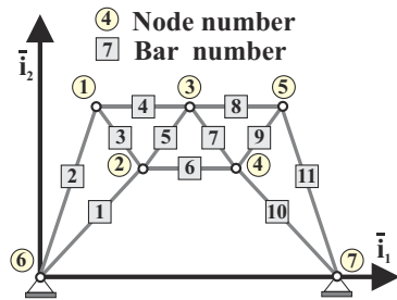
Fig. 10.25. Eleven-bar truss.
