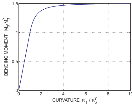
Fig. 13.9. The moment-curvature diagram for a section made of elastic-perfectly plastic material.
