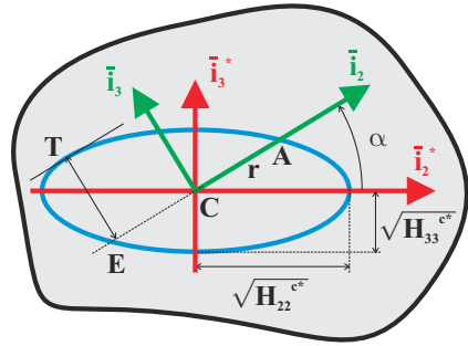
Fig. 6.5. The bending stiffness ellipse of a cross-section.
