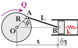
Fig. 9.15. Crank-slider mechanism with a spring.
