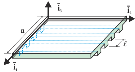
Fig. 16.22. Rectangular plate with directional reinforcement along axis \bar{i}_2 .
