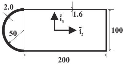
Fig. 8.85. Thin-walled beam cross-section (dimensions in millimeters).
