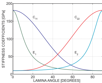
Fig. 2.19. Variation of the stiffness coefficients, C_{11} and C_{22} , and the engineering constants, E_1 and E_2 , as a function of \theta .
