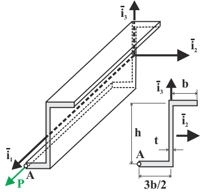
Fig. 6.29. Cantilevered beam with “Z” shaped section under tip axial load.
