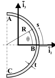
Fig. 8.19. Semi-circular open cross-section.
