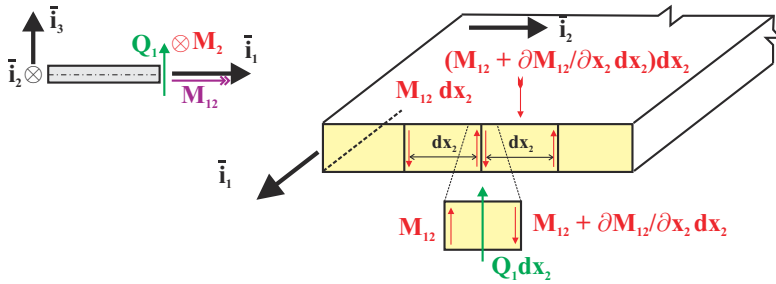
Fig. 16.7. Boundary conditions for free edge.
