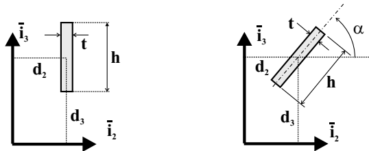
Fig. 6.13. A thin rectangular strip.
