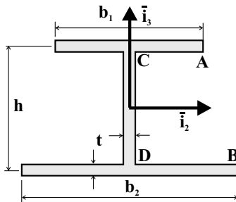
Fig. 8.73. Configuration of the I beam.
