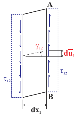
Fig. 15.1. Simplified deformation under shear.
