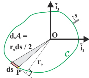
Fig. 8.46. The area of a differential triangle, d\mathcal{A} = 1/2 r_o ds .
