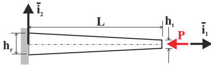
Fig. 14.14. Tapered cantilevered beam under axial load.
