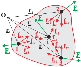
Fig. 9.8. A system of particles.
