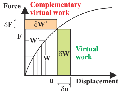
Fig. 9.38. Work and complementary work and their virtual counterparts.
