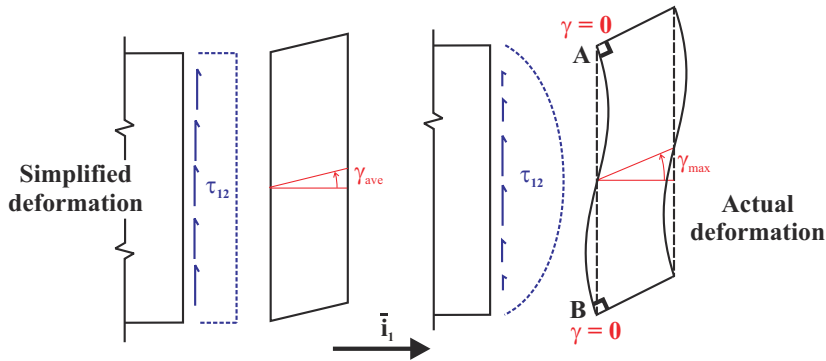
Fig. 15.4. The simplified and actual deformation configurations.
