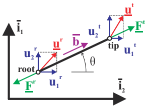
Fig. 9.30. Bar displacements and forces.
