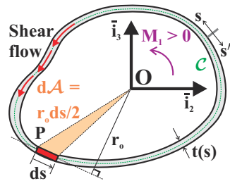
Fig. 8.50. Thin-walled tube of arbitrary cross-sectional shape.
