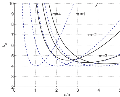
Fig. 16.55. Buckling factor, k_c , versus the plate’s aspect ratio.
