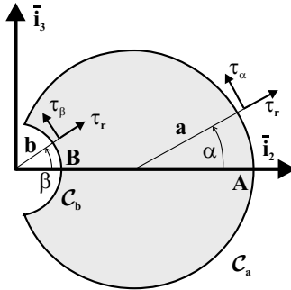
Fig. 7.27. Circular shaft with a circular keyway.
