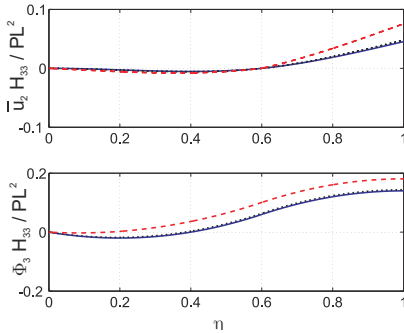
Fig. 15.12. Transverse displacement (top figure) and sectional rotation (bottom figure) of the cantilevered beam with an intermediate support, \alpha = 0.6 . Shear flexibility parameter \bar{s}^2 = 0 , solid line; \bar{s}^2 = 0.0026 , dotted line; \bar{s}^2 = 0.035 , dashed line.
