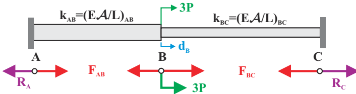
Fig. 4.3. Two bars connected in series with ends fixed.
