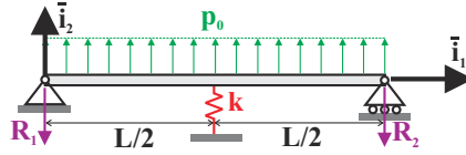
Fig. 10.32. Simply supported beam with a mid-span elastic spring.
