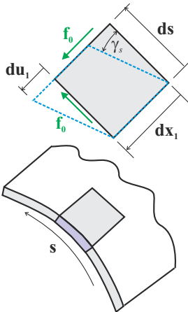
Fig. 8.36. Axial displacement arising from the shear flow f_o .
