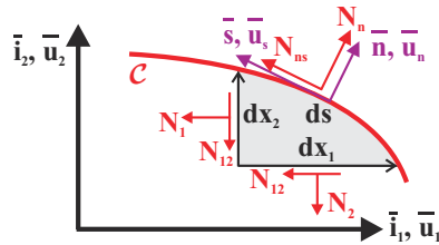
Fig. 16.42. The global coordinate system and the local coordinate system along the edge of the plate.
