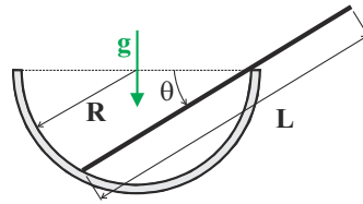
Fig. 10.15. Rod in frictionless hemispherical bowl ( L > 2R ).
