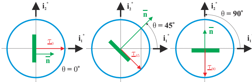
Fig. 1.18. Lamé’s ellipse for the case of pure shear; the three figures illustrate the stress vectors acting on faces at 0, 45, and 90 degrees with respect to axis \bar{i}_1^* .
