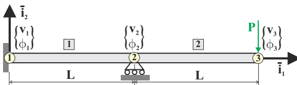
Fig. 11.48. Two-element model of cantilever with mid-span support.
