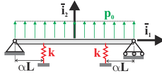
Fig. 11.12. Simply-supported beam with two elastic springs.
