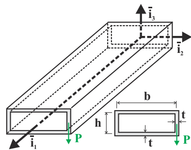
Fig. 8.62. Rectangular box beam subjected to a tip load.
