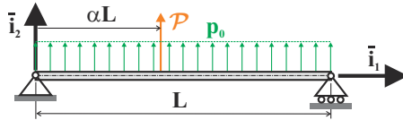
Fig. 10.46. Simply supported beam under uniform loading.
