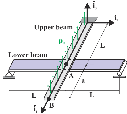
Fig. 11.40. Simply supported beam with cantilever beam crossed and pinned at mid-spans.
