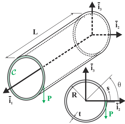
Fig. 8.64. Thin-walled cantilevered beam with circular cross-section under tip transverse load.
