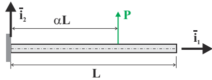
Fig. 15.9. Cantilevered beam with concentrated transverse load.
