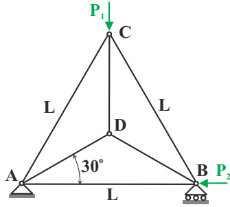
Fig. 9.81. Triangular truss with internal redundancy.
