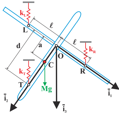
Fig. 9.16. Plan view of the elastically supported aircraft.
