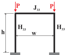
Fig. 14.24. Portal frame subjected to compressive loads.
