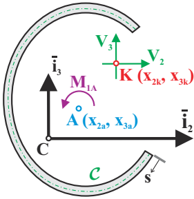
Fig. 8.30. Thin-walled open cross-section subjected to shear forces.
