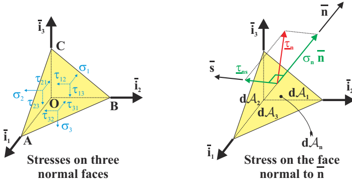
Fig. 1.7. Differential tetrahedron element with one face, ABC , normal to unit vector \underline{n} and the other three faces normal to axes \bar{i}_1 , \bar{i}_2 , and \bar{i}_3 , respectively.
