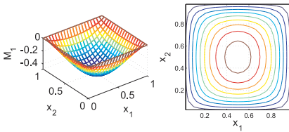
Fig. 16.25. Distribution of bending moment, M_1 , over the plate.
