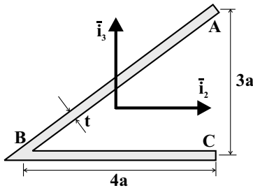
Fig. 8.16. Angled “L” shaped cross-section.
