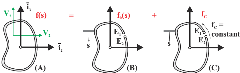
Fig. 8.35. (A): a general closed section. (B): the auxiliary problem created by cutting the section open. (C): the constant closing shear flow.
