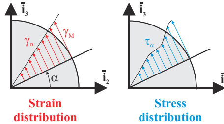
Fig. 13.12. Bar with a circular cross-section undergoing plastic torsion.
