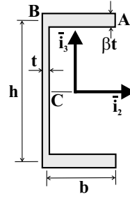
Fig. 8.21. C-channel with variable flange thickness.
