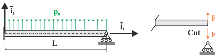
Fig. 5.29. Clamped - simply supported beam under uniform load.
