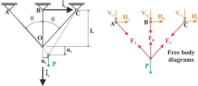
Fig. 9.32. Three-bar truss configuration with free-body diagram.
