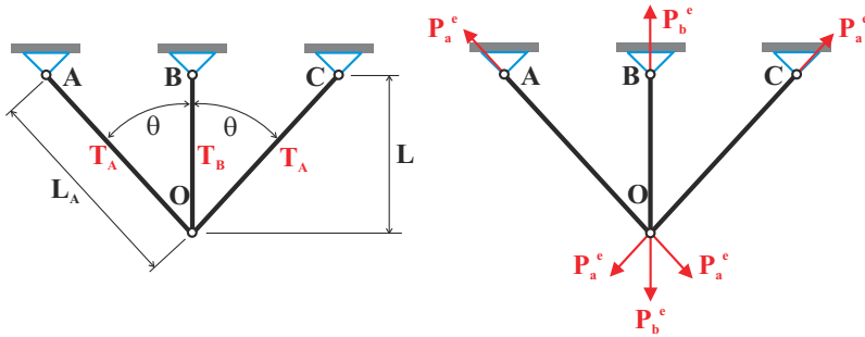
Fig. 13.18. Three-bar truss subjected to temperature changes.
