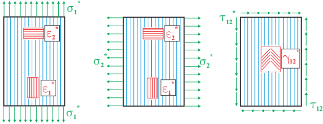
Fig. 2.17. Three simple tests for the determination of the engineering constants.
