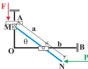
Fig. 9.19. Lever with sliding pivots.
