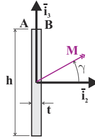
Fig. 6.17. Thin rectangular cross-section.
