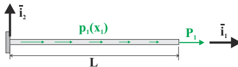
Fig. 11.16. Beam subjected to distributed axial load and tip load.
