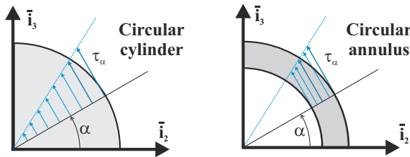
Fig. 7.5. Distribution of circumferential shearing stress over the cross-section.
