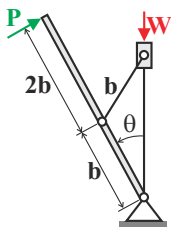
Fig. 9.21. Lever mechanism.
