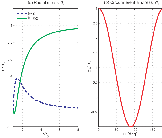
Fig. 3.14. Plots of stress state around circular hole in a thin sheet: (a) \sigma_r/\sigma_a along radii at \theta = 0 and \theta = \pi/2 , and (b) \sigma_\theta/\sigma_a around inside edge of hole.
