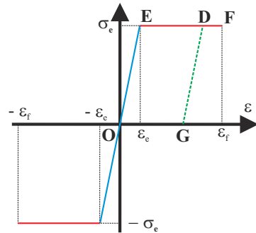
Fig. 2.7. Stress-strain diagram for an elastic-perfectly plastic material.
