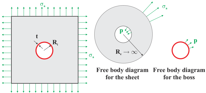
Fig. 3.15. A thin panel with a hole subjected to a biaxial state of stress.
