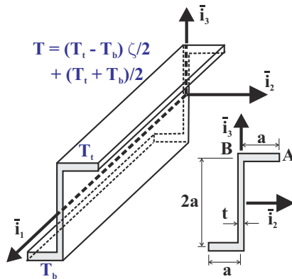
Fig. 13.25. Cantilevered beam subjected to thermal gradient.
