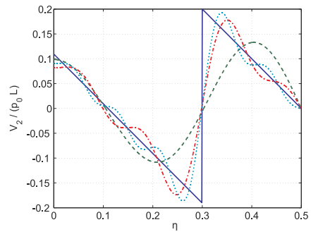
Fig. 11.32. Shear force V_2/(p_0L) for the exact and approximate solutions versus non-dimensional span. Exact solution: solid line; approximate solution case 1: dashed line, case 2: dash-dotted line, case 3: dotted line.
