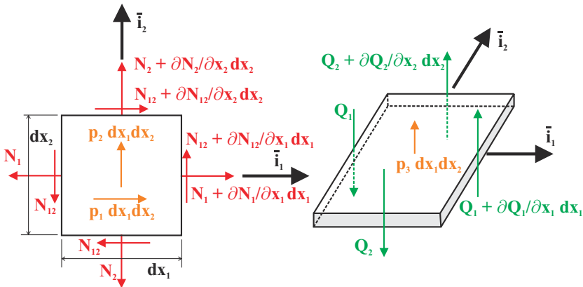
Fig. 16.4. Left figure: free body diagram for the equilibrium of in-plane forces. Right figure: free body diagram for the equilibrium of transverse shear forces.
