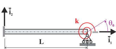
Fig. 5.37. Cantilevered beam with tip torsional spring.
