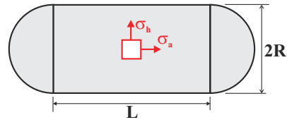
Fig. 1.20. Stresses acting in a pressure vessel.
