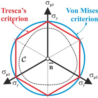
Fig. 13.2. View of the geometric stress space from along unit vector \bar{n} ; the octahedral face is in the plane of the figure.
