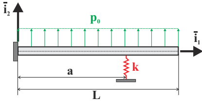
Fig. 11.41. Cantilever beam with uniform load and spring at intermediate point.
