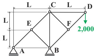
Fig. 9.47. Planar truss with tip load.
