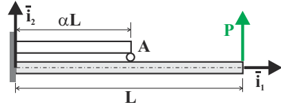
Fig. 15.18. Cantilevered beam with intermediate support.
