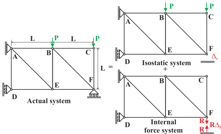
Fig. 9.68. Calculation of member forces in a 2-bay truss with a redundant support.
