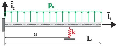
Fig. 10.34. Cantilevered beam with intermediate spring support.
