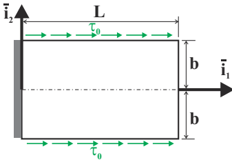
Fig. 12.7. Upper panel of a box beam subjected to edge shear forces.
