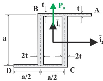
Fig. 6.27. Box-Z shaped cross-section.
