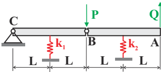
Fig. 9.25. Two articulated bars supported by springs.
