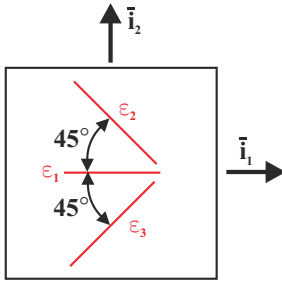
Fig. 16.21. Configuration of the three strain gauges at the upper surface of the plate.
