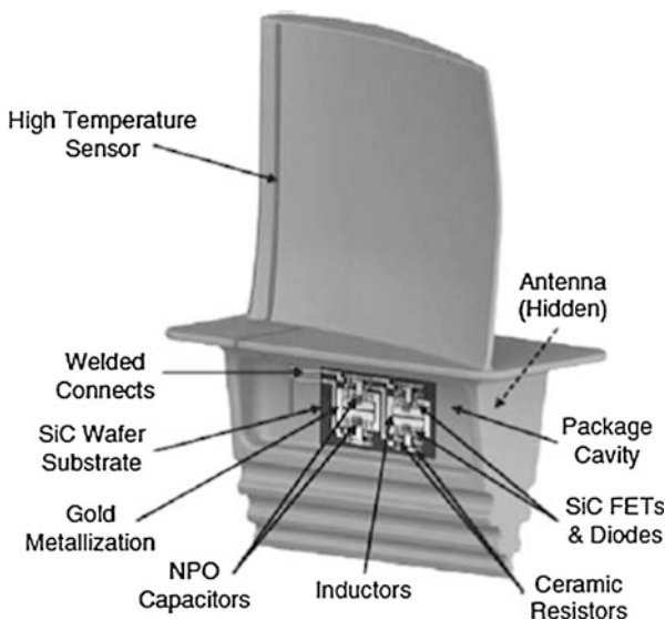
Fig. 11.12 A direct write sensor and associated wiring on a turbine blade structure. Signal conditioning electronics are positioned on a more shielded spot (Courtesy MesoScribe Technologies, Inc. and Arkansas Power Electronics Int.)
