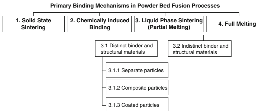
Fig. 5.5 Primary binding mechanisms in powder bed fusion processes (adapted from [1])
