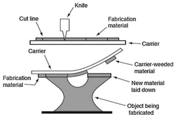
Fig. 9.3 Offset Fabbing system, Ennex Corp ( http://www.ennex.com/fab/Offset/ )
