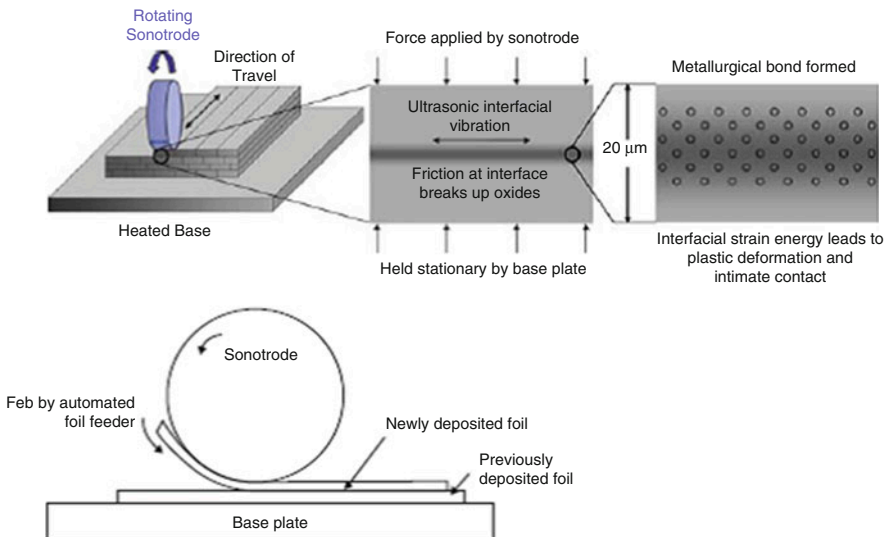
Fig. 9.7 Schematic of ultrasonic consolidation
