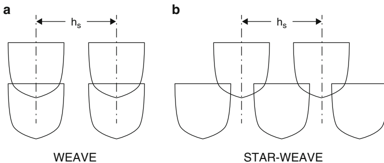
Fig. 4.10 Cross-sectional view of WEAVE and STAR-WEAVE patterns
