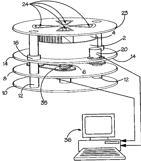
Fig. 8.2 Schematic of a spiral growth manufacturing BJ machine
