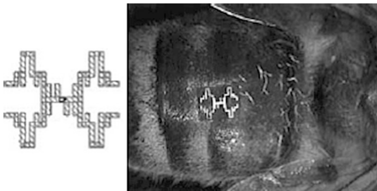
Fig. 11.11 35-GHz fractal antenna design ( left ) and MAPLE-DW printed antenna on the abdomen of a dead drone honeybee ( right ). (Courtesy Douglas B. Chrisey)
